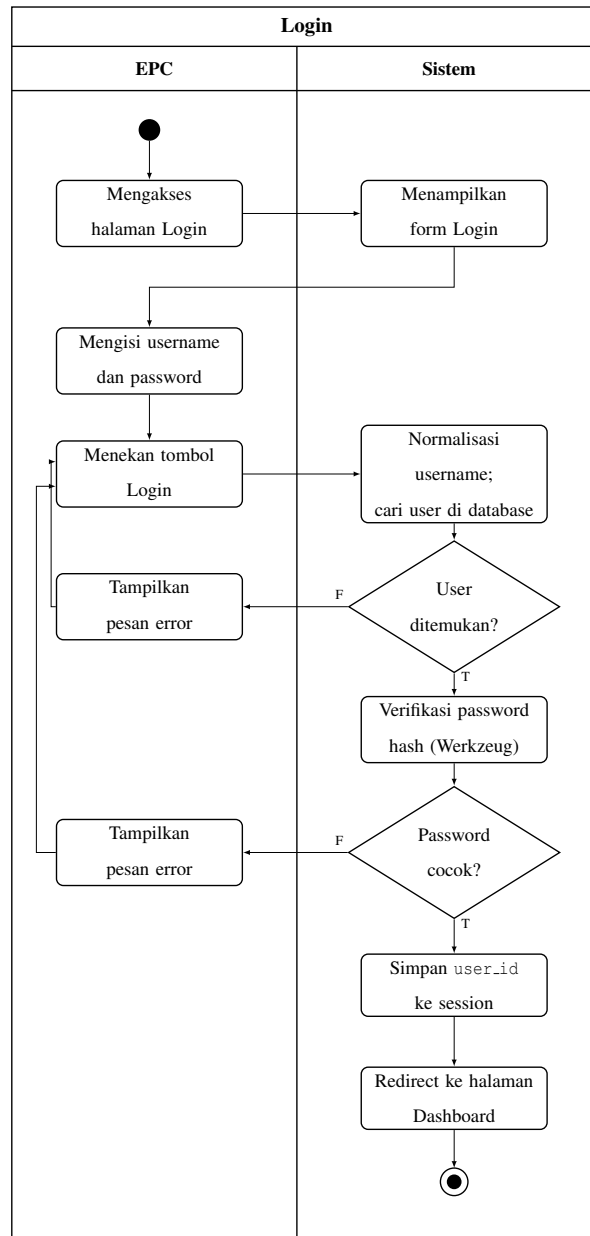
Gambar 3.3. Activity Diagram Login
