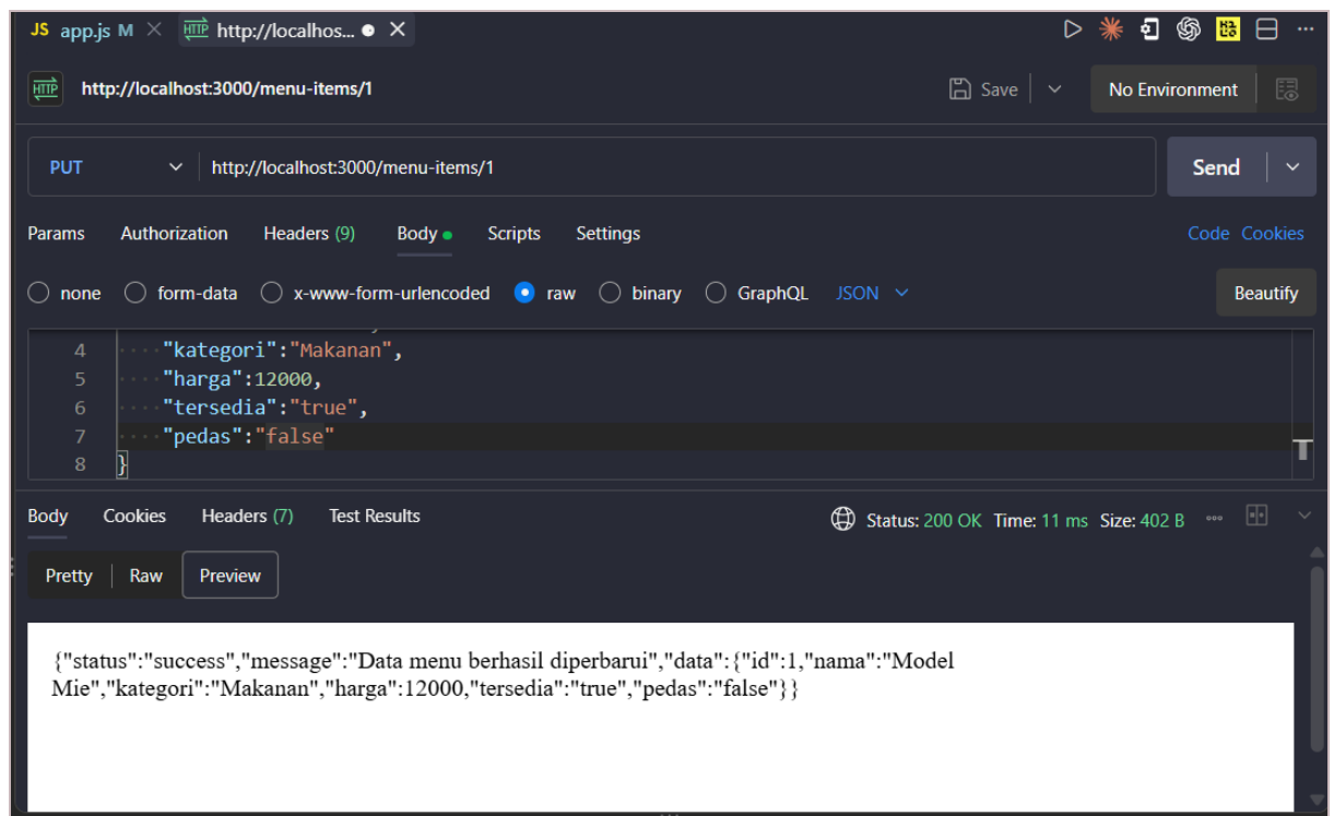
Gambar 7. PUT http://localhost:3000/menu-items/1
