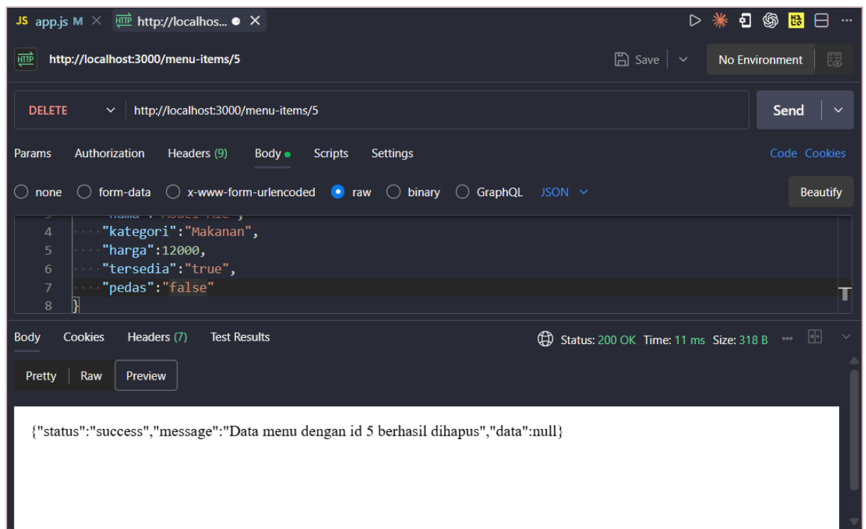
Gambar 9. DELETE http://localhost:3000/menu-items/5
