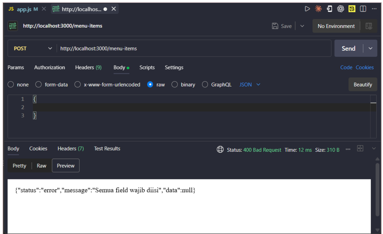
Gambar 6. POST http://localhost:3000/menu-items
