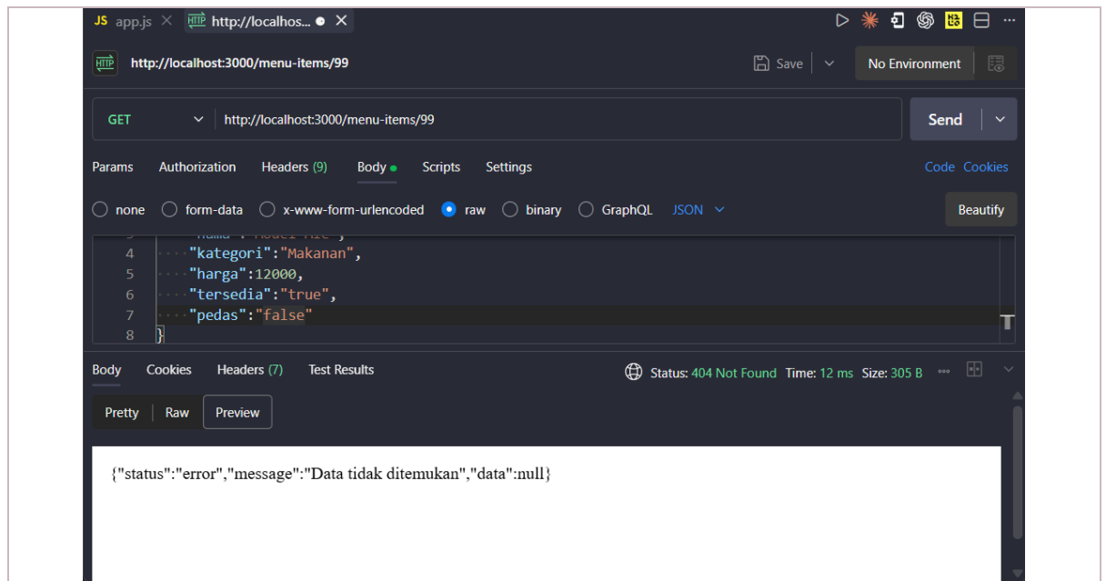
Gambar 3. GET http://localhost:3000/menu-items/99
