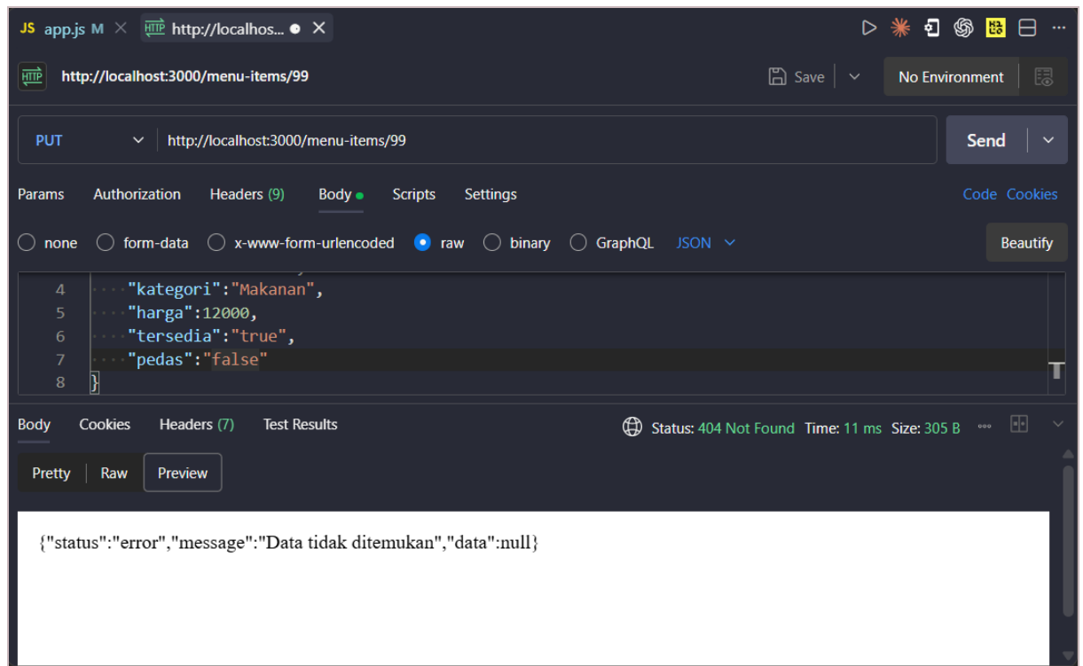
Gambar 8. PUT http://localhost:3000/menu-items/99
