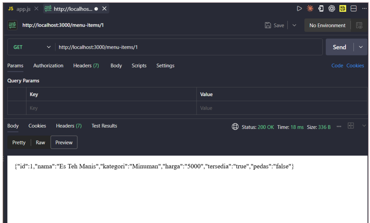
Gambar 2. GET http://localhost:3000/menu-items/1
