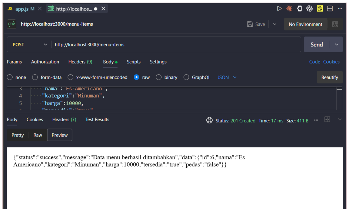
Gambar 5. POST http://localhost:3000/menu-items
