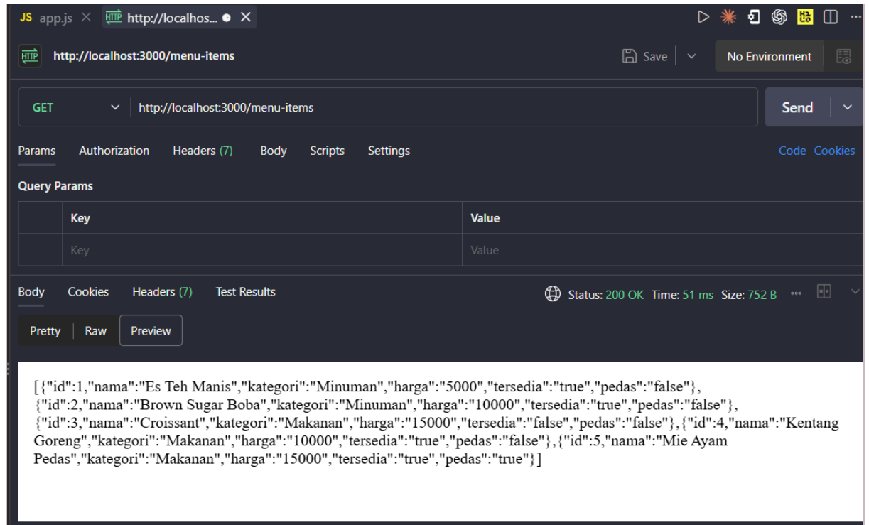
Gambar 1. GET http://localhost:3000/menu-items
