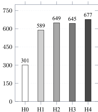
(c) Occupied slices
