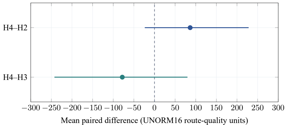
Figure 4.3. Paired mean route-quality differences with registered percentile 95% confidence intervals. Both intervals cross zero; the line at zero denotes no mean difference.
