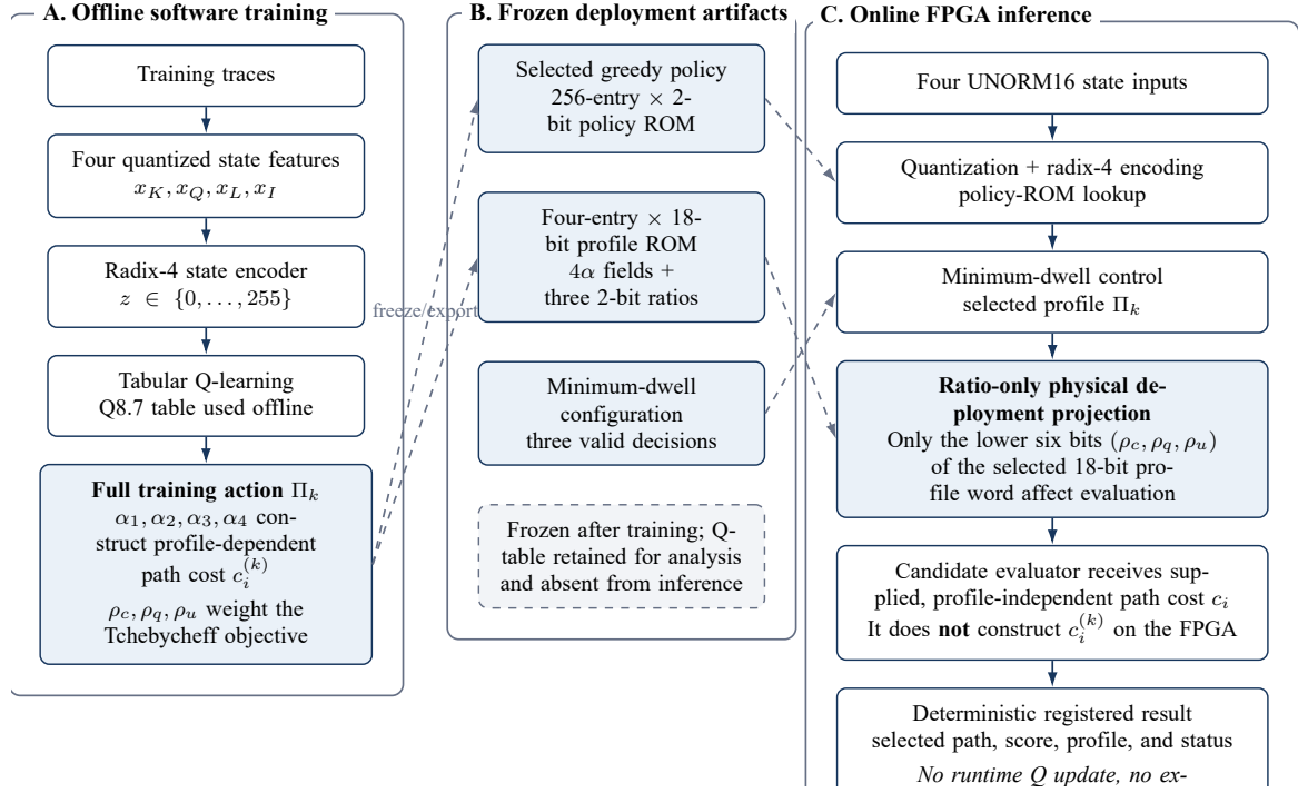
Figure 3.4. Offline training and FPGA deployment path. Software training uses the complete profile action: coefficients \alpha_1 – \alpha_4 construct profile-dependent path cost and ratios (\rho_c, \rho_q, \rho_u) weight the Tchebycheff objective. The physical implementation deploys the frozen state-to-profile policy, minimum-dwell control, and only the objective-ratio projection over externally supplied profile-independent path cost; it performs no runtime Q update, exploration, on-chip learning, or on-FPGA construction of c_i^{(k)} .
