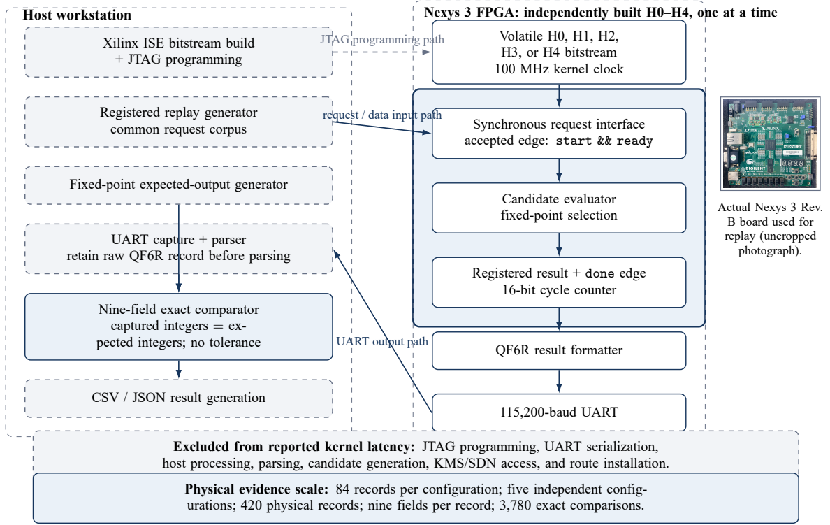
Figure 3.6. Physical replay and exact-comparison setup. Each independently implemented H0–H4 bitstream was programmed on the same Nexys 3 board, replayed with the common request corpus, captured through UART, and compared field-by-field with the fixed-point reference; the inset is the uncropped photograph of the board used. Only the accepted-request-to-done interval inside the solid FPGA kernel boundary contributes to reported kernel latency. Dashed host and transport functions, including programming, serialization, parsing, candidate generation, KMS/SDN access, and route installation, are excluded.
