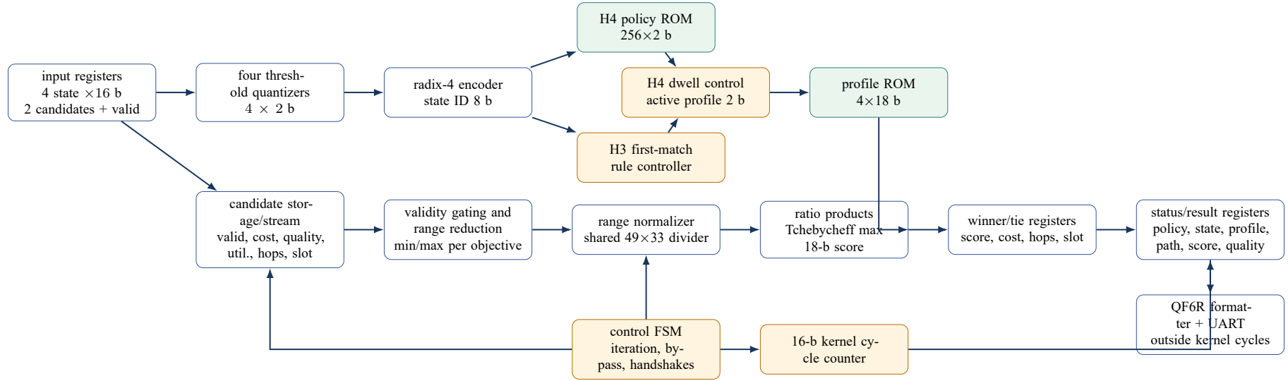
Figure 3.2. Detailed QFlow RTL architecture. H0 bypasses the profile and iterative score path; H1 bypasses profile-ROM lookup; H2 fixes \Pi_0 ; H3 uses the rule controller; H4 uses policy ROM and dwell control. Formatter and UART time are not included in the kernel-cycle measurement.
