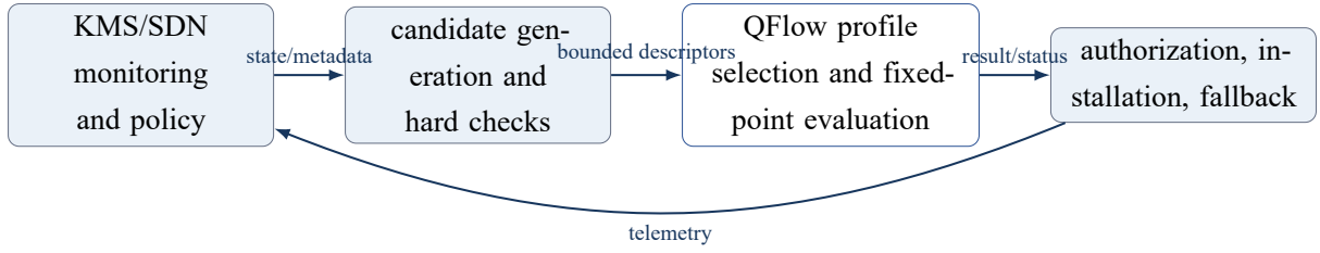
Figure 3.1. System boundary. Only profile selection and candidate evaluation are included in the measured FPGA kernel.
