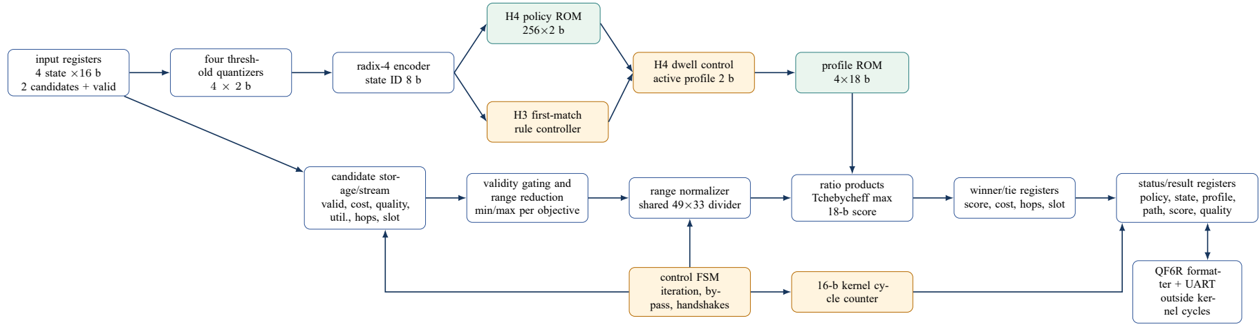
Figure 3.2. Detailed QFlow RTL architecture. H0 bypasses the profile and iterative score path; H1 bypasses profile-ROM lookup; H2 fixes \Pi_0 ; H3 uses the rule controller; H4 uses policy ROM and dwell control. Formatter and UART time are not included in the kernel-cycle measurement.
