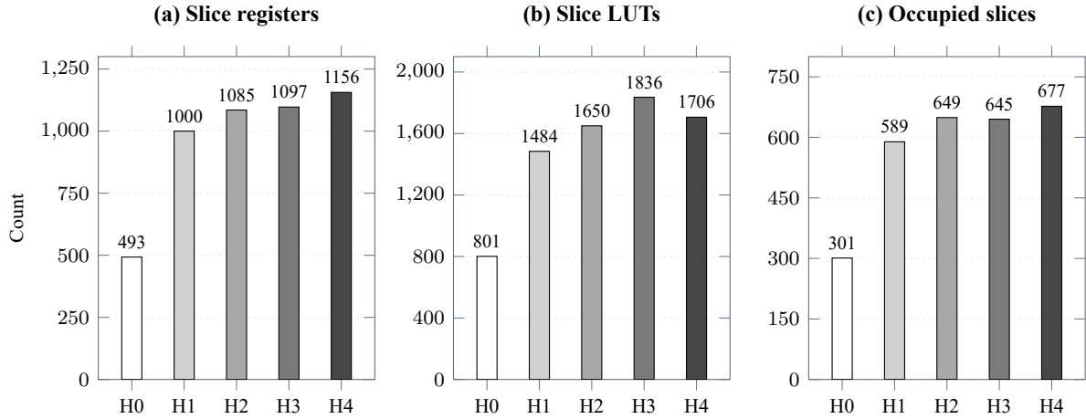
Figure 4.5. Post-route FPGA resource utilization for the five independent configurations. The aligned, zero-based panels report exact slice-register, slice-LUT, and occupied-slice counts from Table 4.5; grayscale shade identifies H0 through H4 consistently in each panel. H4 mapped to fewer LUTs than H3 but used more registers and occupied slices, so individual resource categories and physical slice packing need not move in the same direction.
