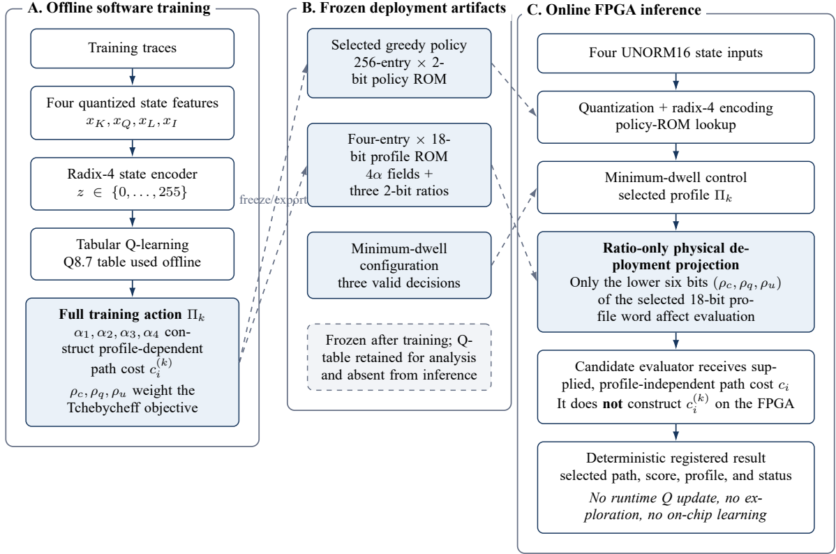
Figure 3.4. Offline training and FPGA deployment path. Software training uses the complete profile action: coefficients \alpha_1 – \alpha_4 construct profile-dependent path cost and ratios ( \rho_c, \rho_q, \rho_u ) weight the Tchebycheff objective. The physical implementation deploys the frozen state-to-profile policy, minimum-dwell control, and only the objective-ratio projection over externally supplied profile-independent path cost; it performs no runtime Q update, exploration, on-chip learning, or on-FPGA construction of c_i^{(k)} .
