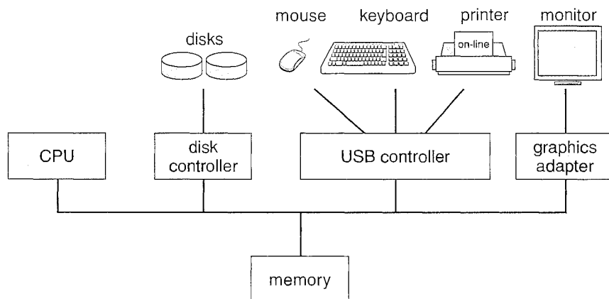
Figure 19.1 Bus-oriented organization.
