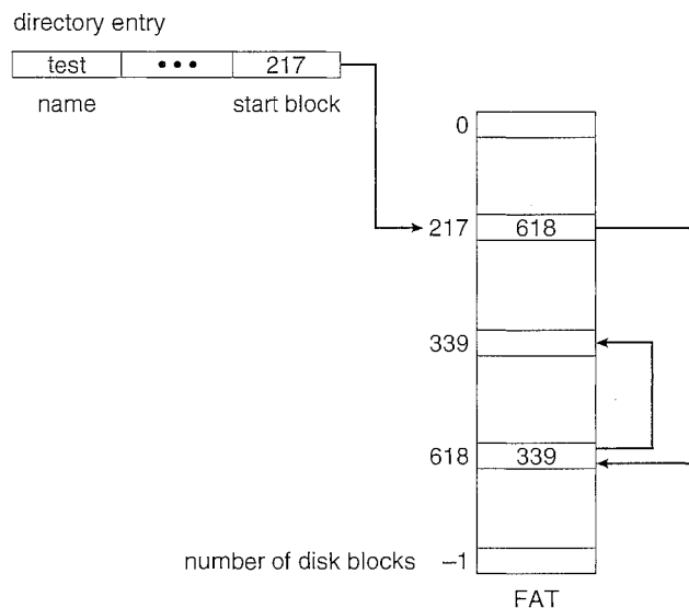
Figure 11.7 File-allocation table.
