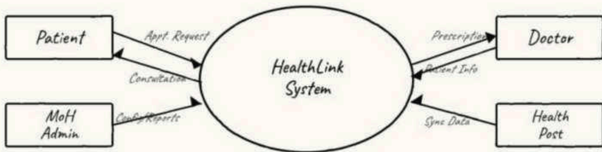
Fig: DFD Level-0 for HealthLink System
