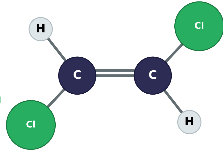
Trans isomer
