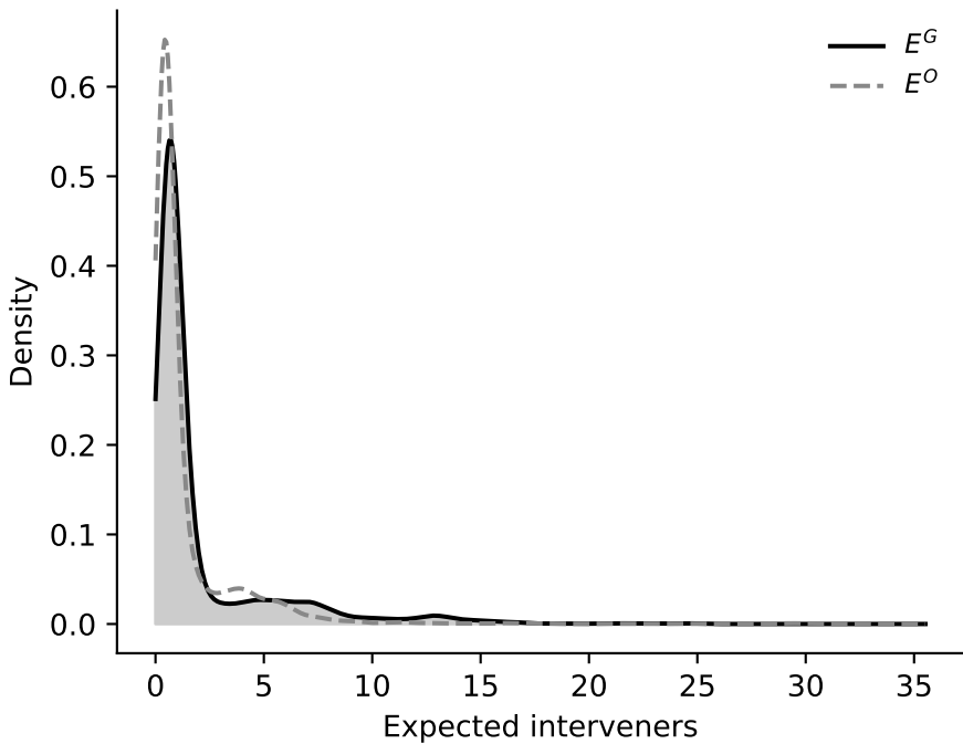
Distribution of E^G and E^O (all country-years)
