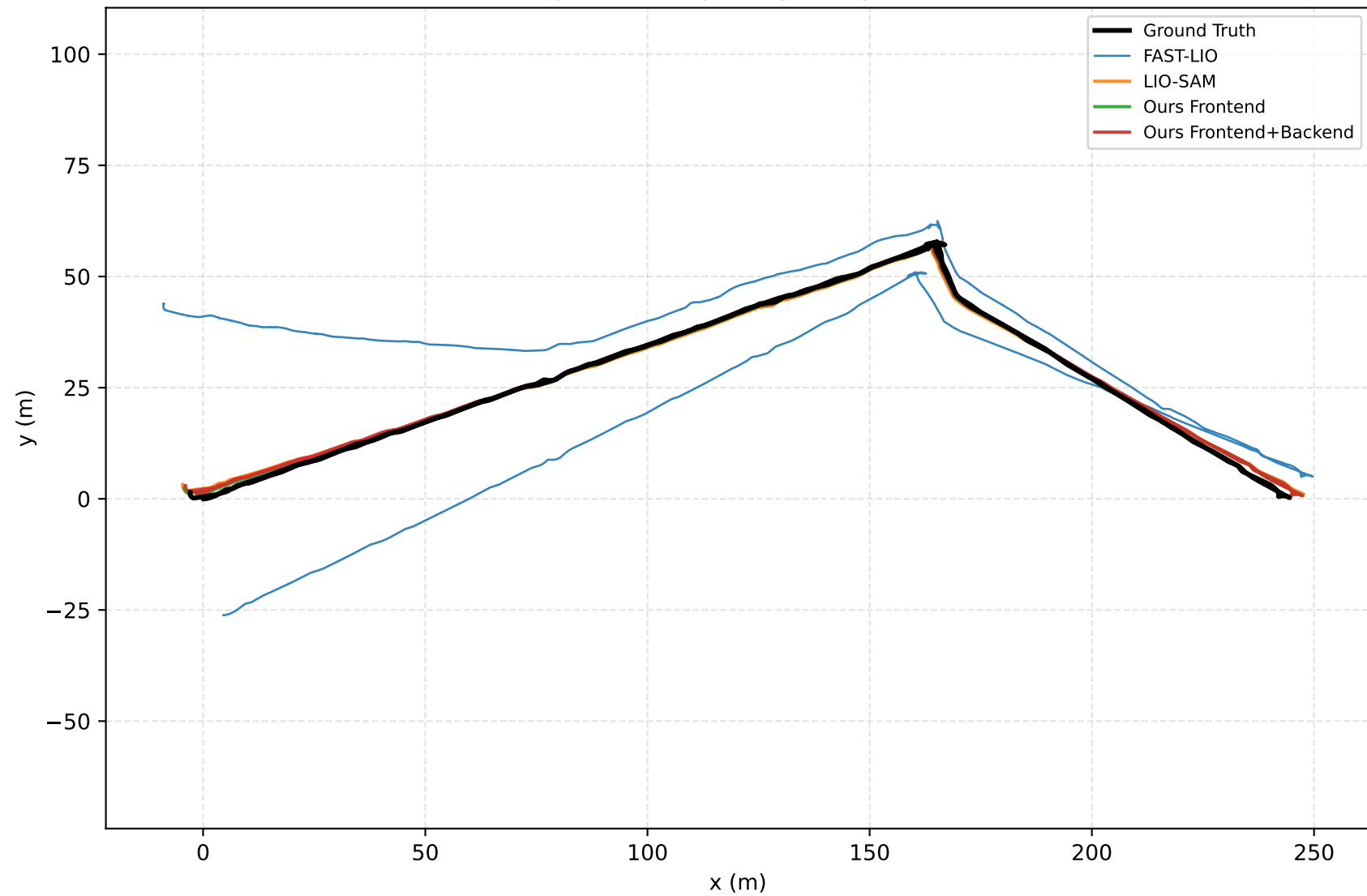
Aligned XY Trajectory Comparison
