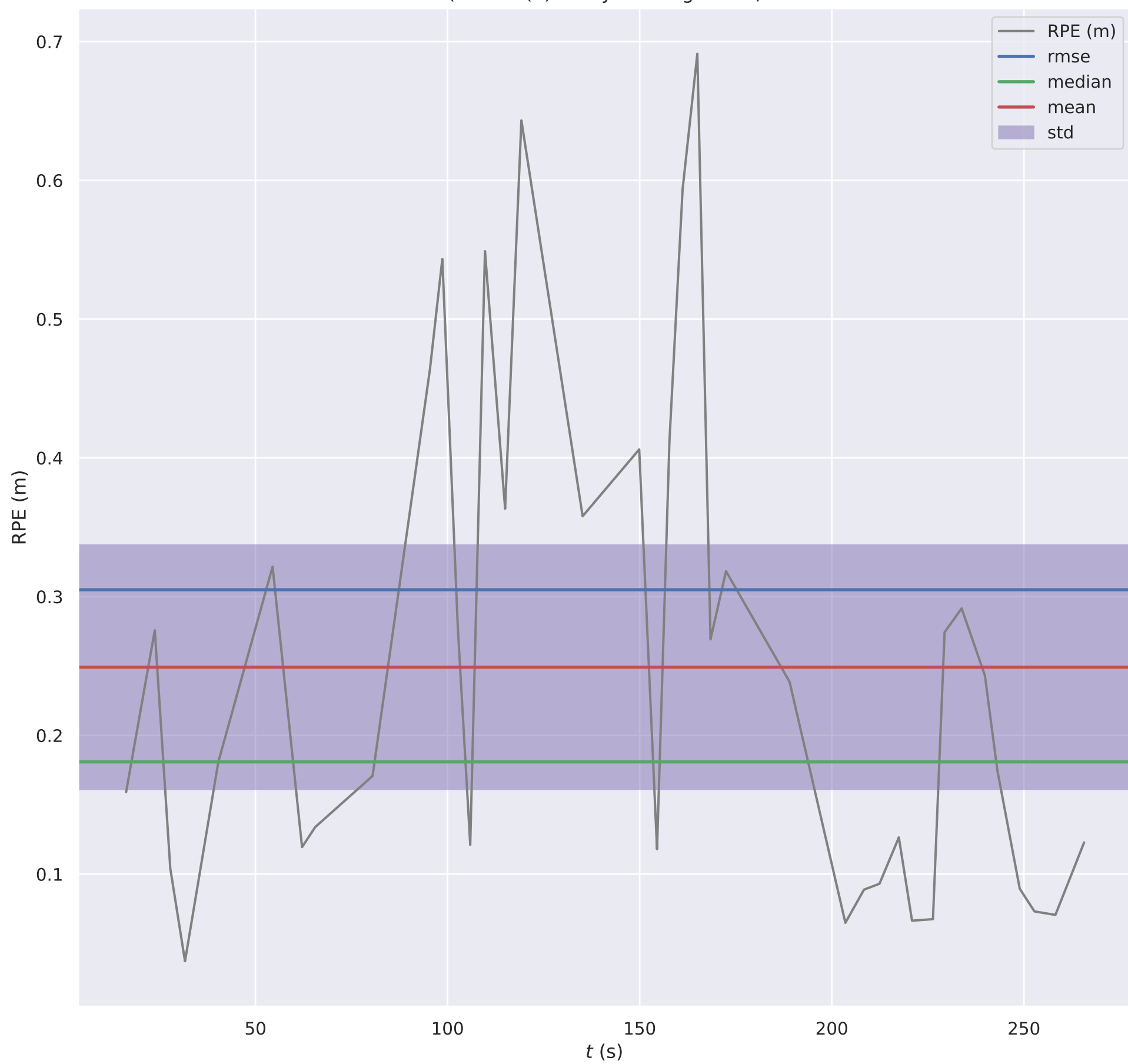
RPE w.r.t. translation part (m) for \delta = 10.0 (m) using consecutive pairs (with SE(3) Umeyama alignment)
