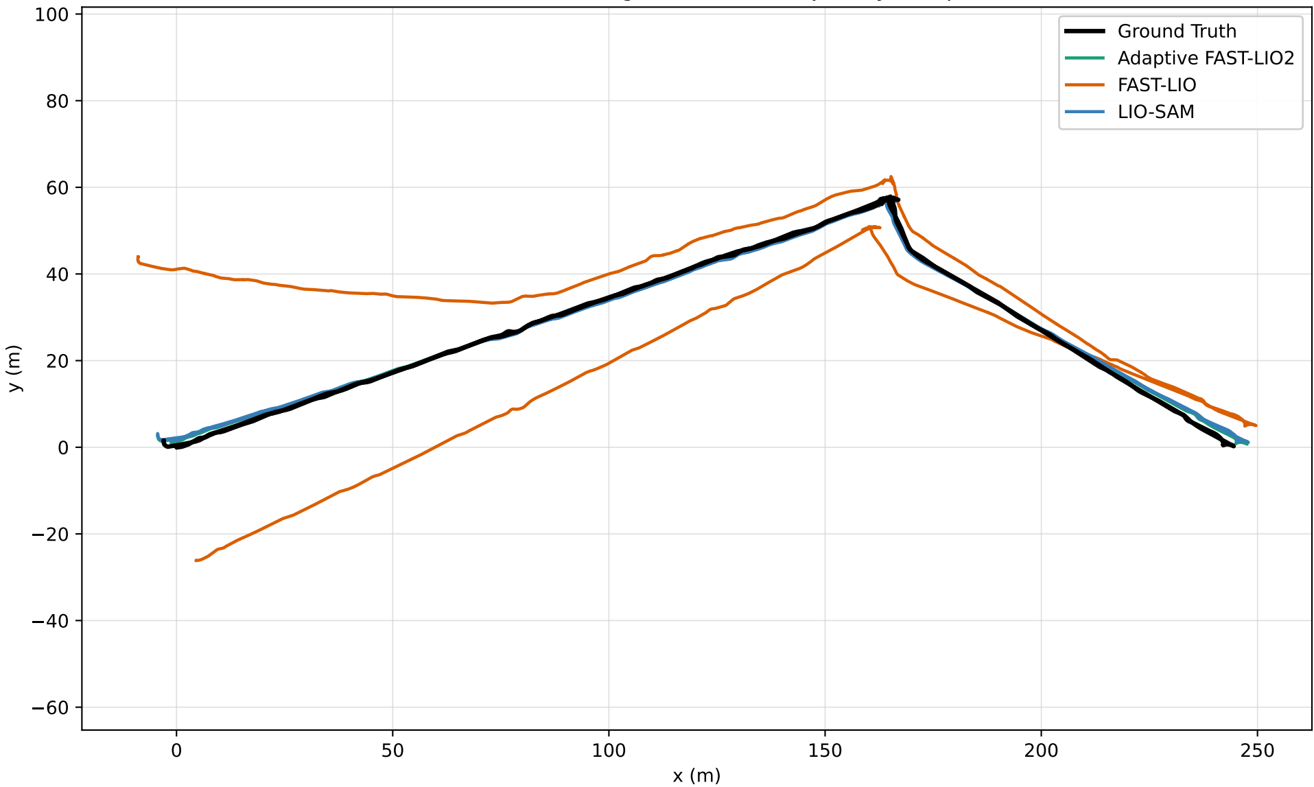
SubT-MRS Hawkins Long Corridor: XY Trajectory Comparison
