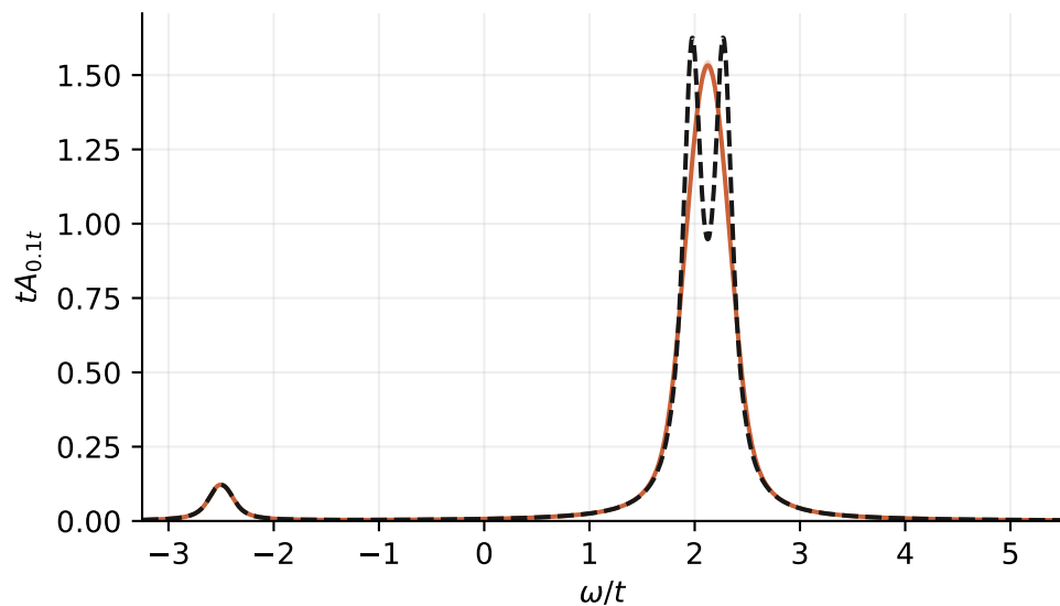
Broad continuum
