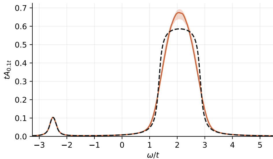
Broad continuum
