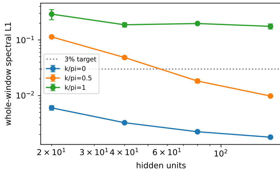
Finite ED calibration: \eta=0.05 , metric cutoff= 1e-10 ; two-seed range
