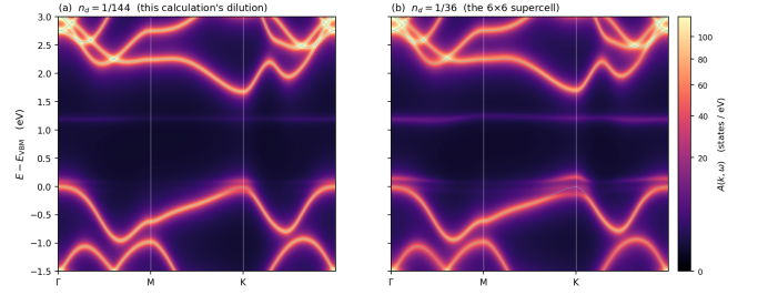
FIG. 1. Electron-defect spectral function A(\mathbf{k}, \omega) along \Gamma –M–K– \Gamma for the relaxed sulfur vacancy, at two concentrations, with the bare interpolated bands overlaid. The flat in-gap lines are the Koster–Slater bound states; their energy is \mathbf{k} -independent by construction while their weight is not.
