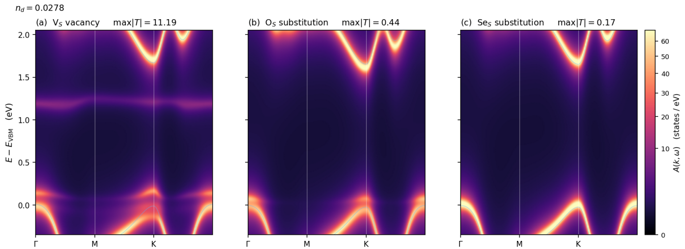
FIG. 2. The same pipeline applied to three point defects at n_d = 1/36 : identical chains (16 blocks, 141 min), identical transform, identical cluster. A bound state requires 1 - \mathcal{V}\mathcal{G}^A to become singular in the gap, where \mathcal{G}^A is real; only the vacancy achieves it. The isovalent substitutions leave the gap clean and merely broaden the host bands, strongly for \text{O}_S and barely at all for \text{Se}_S .
