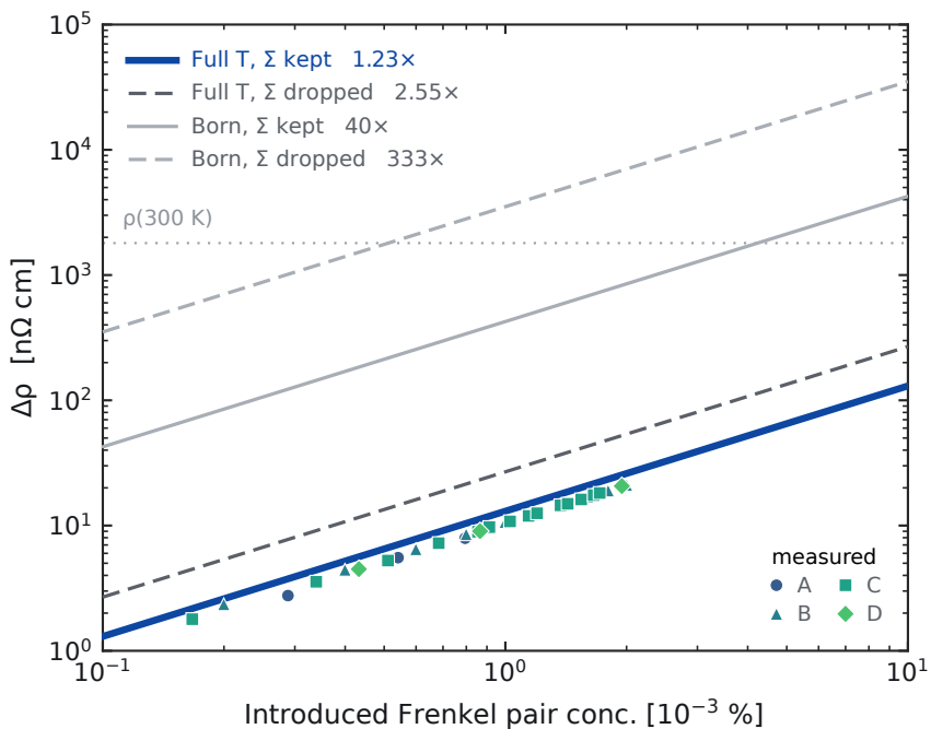
points: electron-irradiation data of Sunko et al., Phys. Rev. X 10, 021018 (2020), FIG. 10, PtCoO 2 samples A-D; ratios are to the measured slope, 10.5 \text{n}\Omega\text{ cm} per 10^{-3}\%
