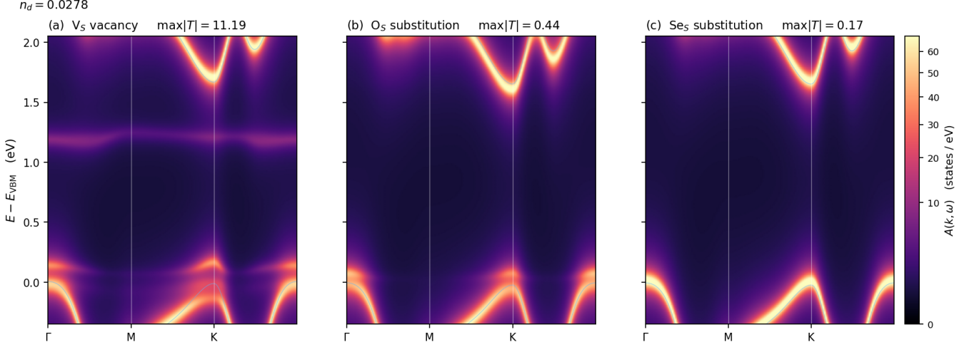
FIG. 2. The same pipeline applied to three point defects at n_d = 1/36 : identical chains (16 blocks, 141 min), identical transform, identical cluster. A bound state requires 1 - \mathcal{V}\mathcal{G}^A to become singular in the gap, where \mathcal{G}^A is real; only the vacancy achieves it. The isovalent substitutions leave the gap clean and merely broaden the host bands, strongly for O_S and barely at all for Se_S .
