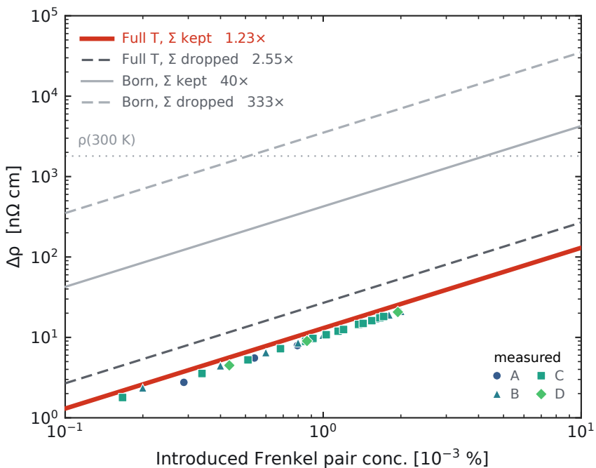
points: electron-irradiation data of Sunko et al., Phys. Rev. X 10, 021018 (2020), FIG. 10, PtCoO 2 samples A-D; ratios are to the measured slope, 10.5 nΩ cm per 10^{-3} %
