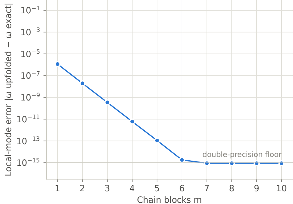
Light defect: the local mode converges in a few blocks
