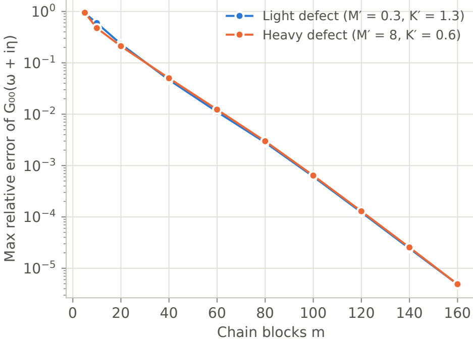
In-band response: error falls as the chain grows
