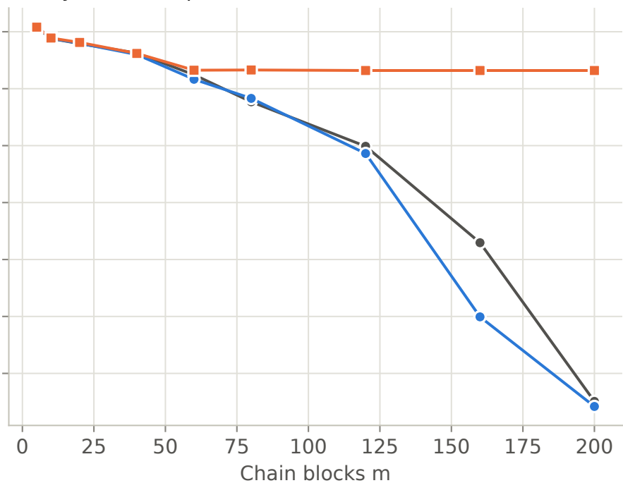
Heavy defect: in-plane G at the defect
