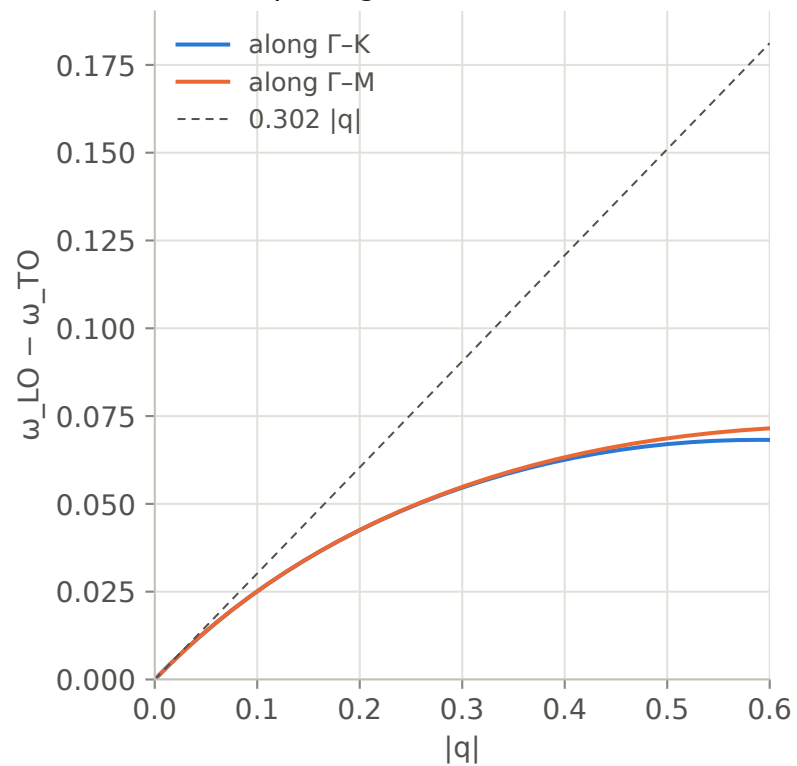
LO-TO splitting near \Gamma
