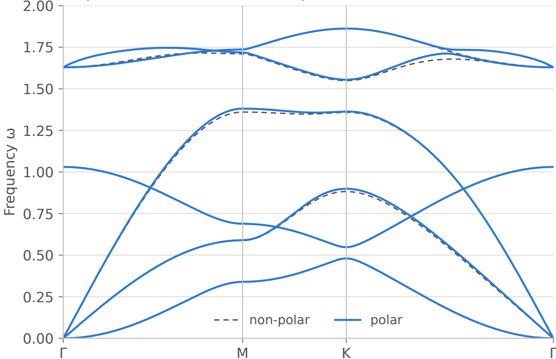
Dispersion with and without the polar term
