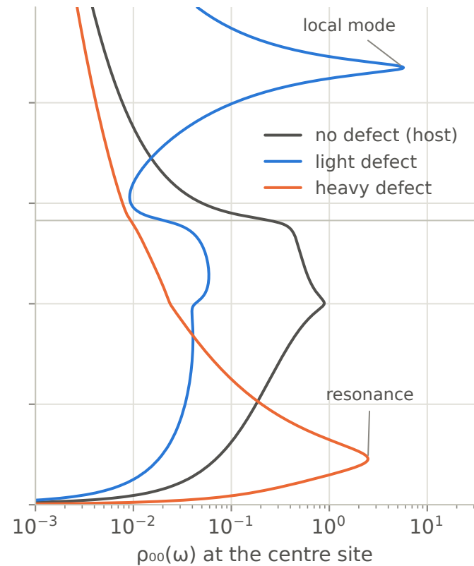
Local density of states
