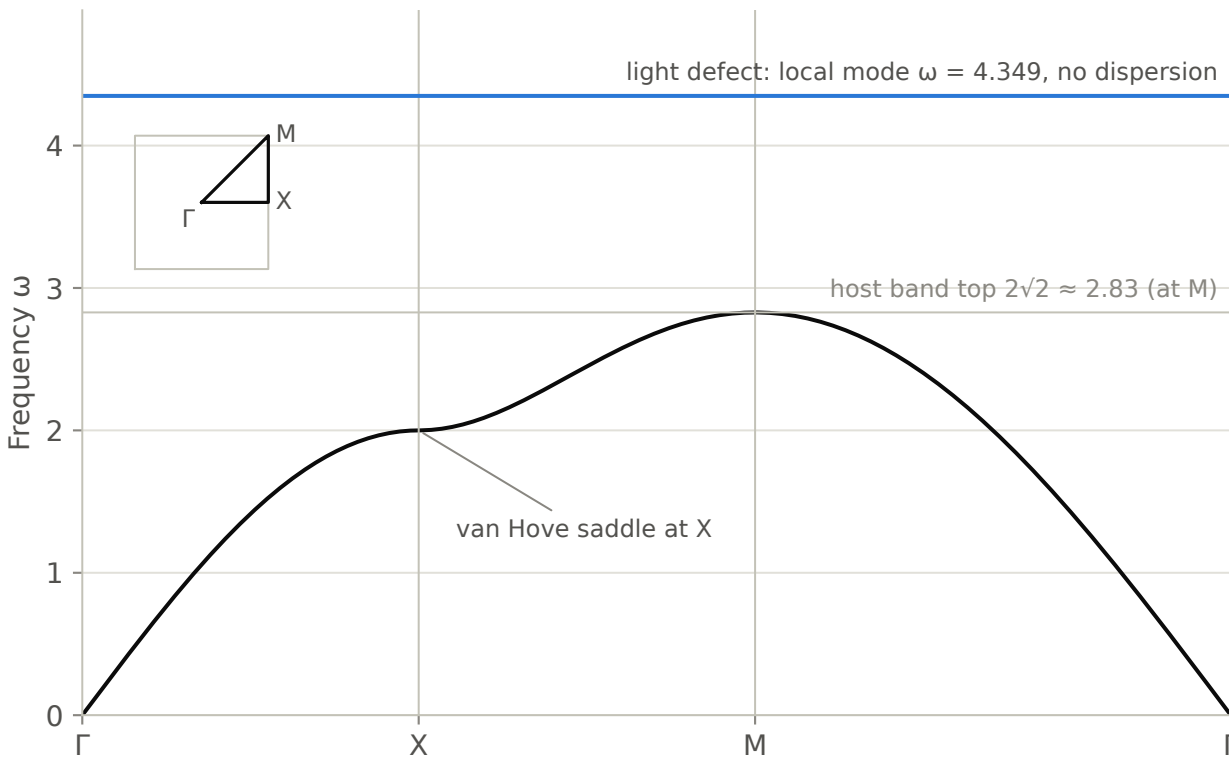
Host phonon dispersion
