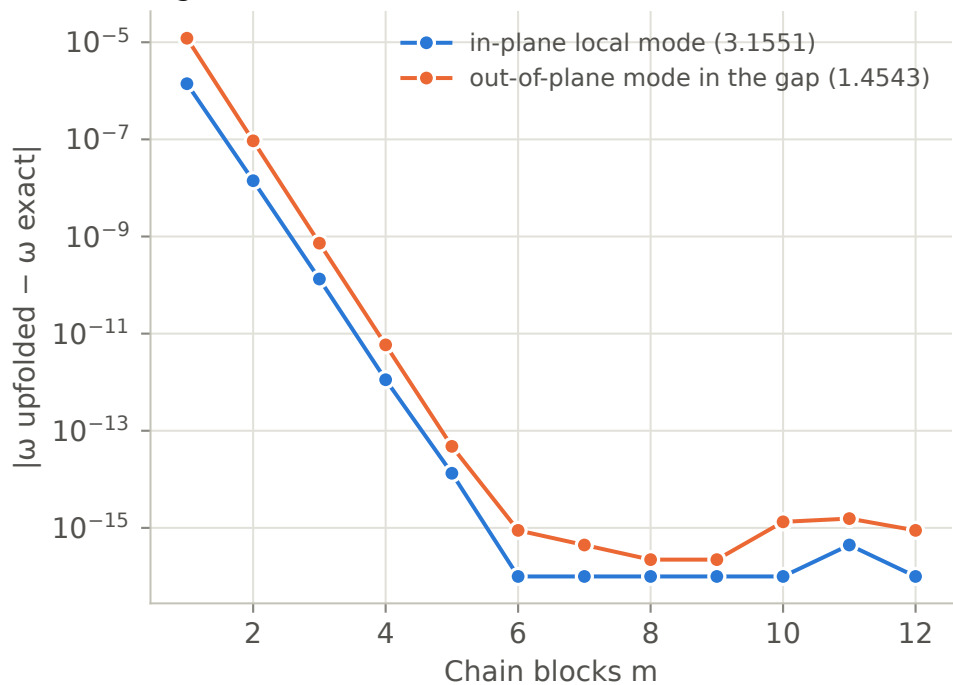
Light defect: bound states
