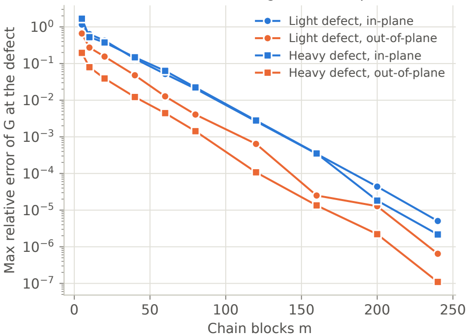
Defect-site Green function against the supercell
