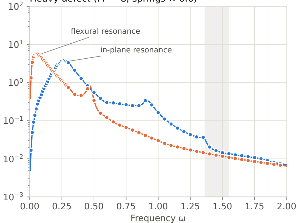
Heavy defect ( M' = 8 , springs \times 0.6 )
