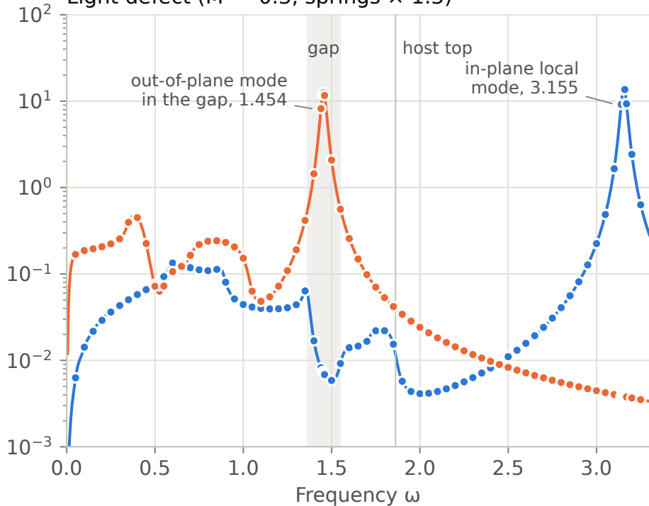
Light defect ( M' = 0.3 , springs \times 1.3 )
