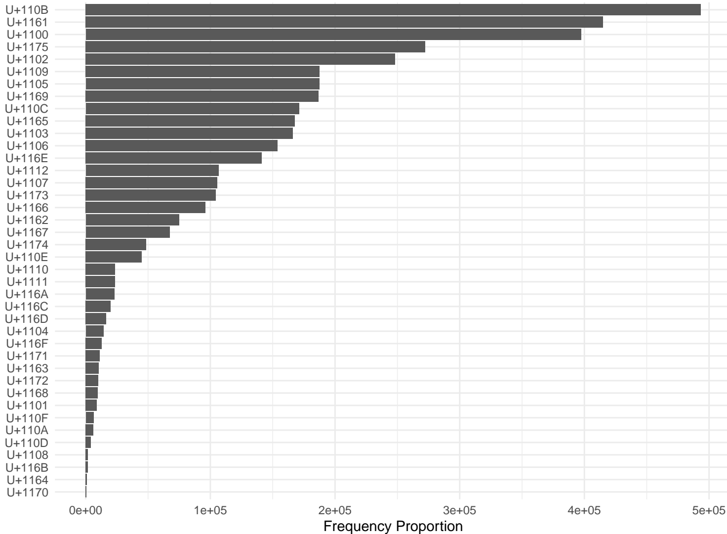
Unicode Frequency (Weighted by Word Frequencies)
