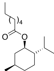
fast-reacting enantiomer of menthyl heptanoate
