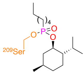
inactivated lipase mimics transition state
