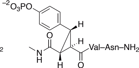
6.2 , K_D = 0.36 \mu\text{M}
