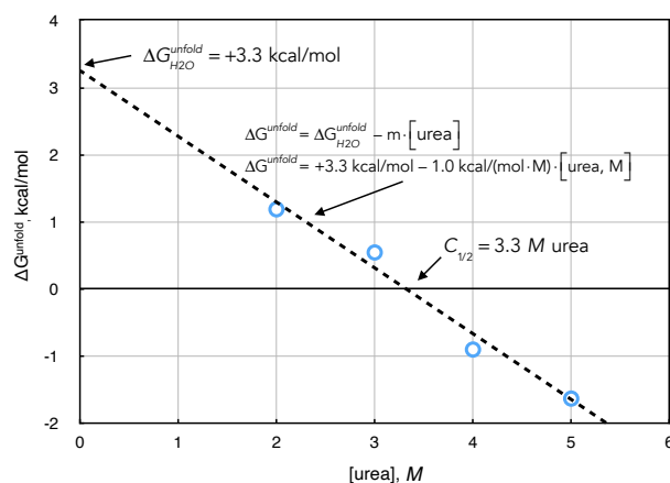
Figure 5.23. Linear extrapolation plot of the data from Table Table 5.5 above. The best fit line to the data is \Delta G^{unfold} = 3.3 - 1.0 \cdot [\text{urea}] , which indicates that \Delta G_{H_2O}^{unfold} is 3.3 kcal/mol.
