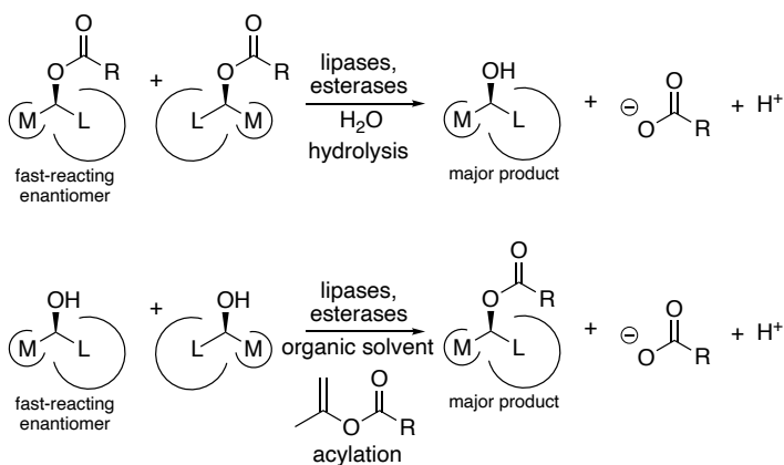
Figure 8.15. The rule for secondary alcohols. M is a medium-sized substituent such as methyl; L is a large substituent such as phenyl. The top reaction is a hydrolysis of a racemic ester in water. The bottom reaction is an acylation of an alcohol in an organic solvent. In both cases the ester or alcohol with the large substituent on the right reacts faster.
