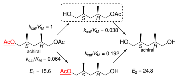
Figure 8.20. Enhancement of stereoselectivity during the desymmetrization of (2R,4S)-2,4-dimethylpentane-1,5-diyl diacetate catalyzed by porcine pancreatic lipase to form (2R,4S)-5-hydroxy-2,4-dimethylpentyl acetate (in box). Both steps favor hydrolysis of the acetate underlined and in red text with similar enantioselectivity: E_1 = 15.6 , E_2 = 24.8 . If only step 1 occurred (diacetate to monoacetate), then the overall enantioselectivity would be 15.6 and the product would have 88% ee. At low conversion (<50% yield of monoacetate), the product has ~88% ee. As the reaction continues the second step (monoacetate to diol) selectively converts the minor enantiomer to diol and enhances the enantiomeric purity to 97% ee at 70% yield of monoacetate.
