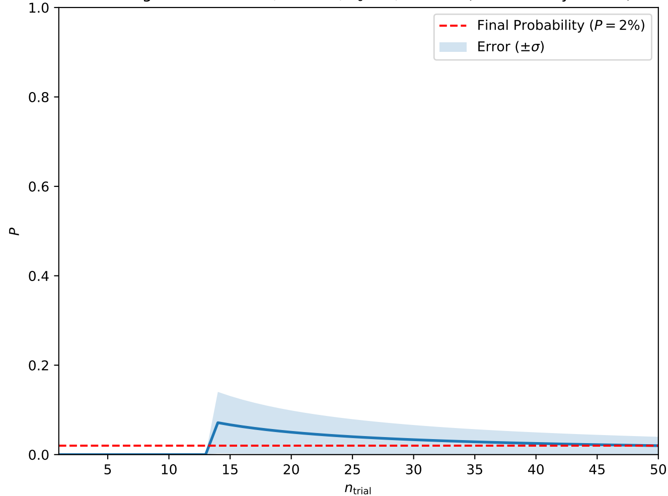
Convergence at A = 0.7, H = 0.3, T_0 = 1, w = 2.5 (Isolated Skyrmions)
