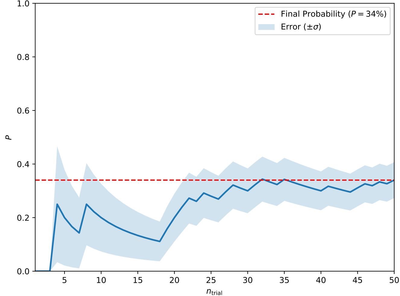
Convergence at A = 0.7, H = 0.3, T_0 = 1, w = 5 (Isolated Skyrmions)
