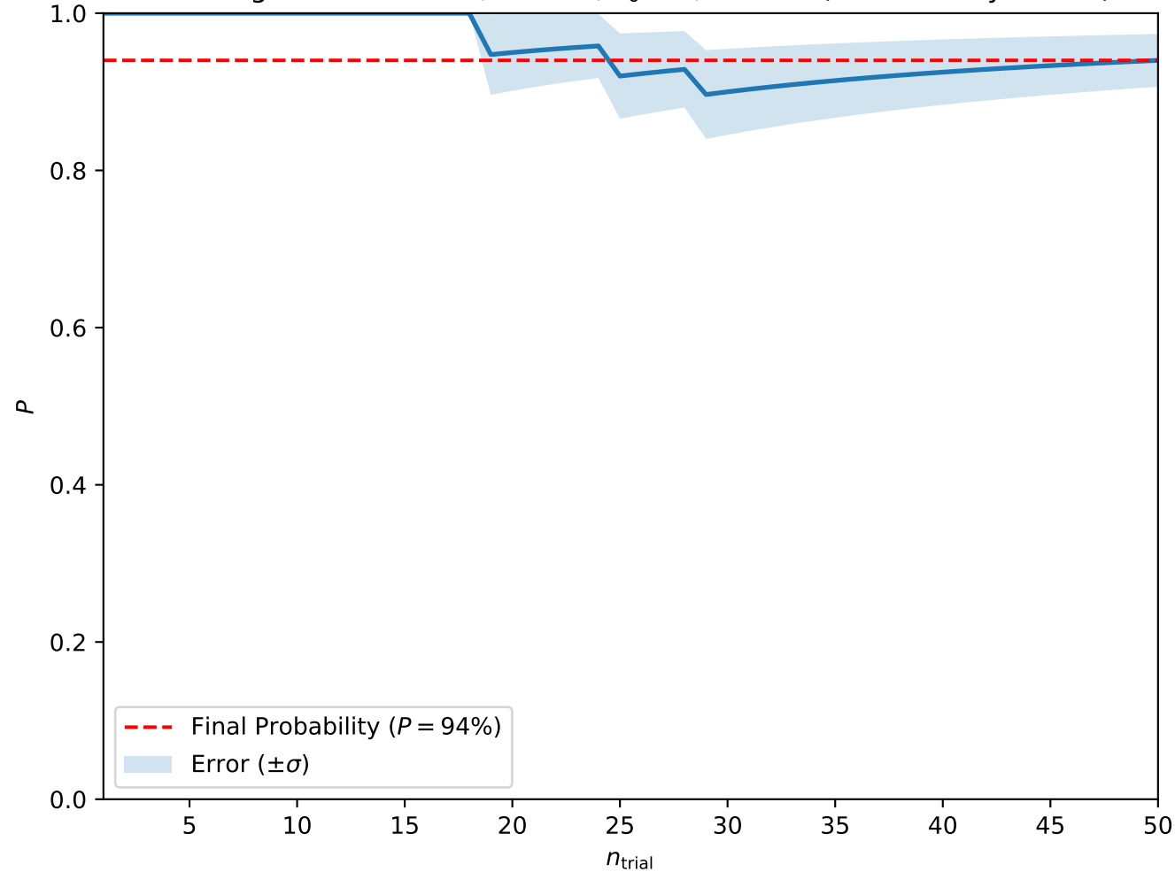
Convergence at A = 0.7, H = 0.3, T_0 = 1, w = 7.5 (Isolated Skyrmions)
