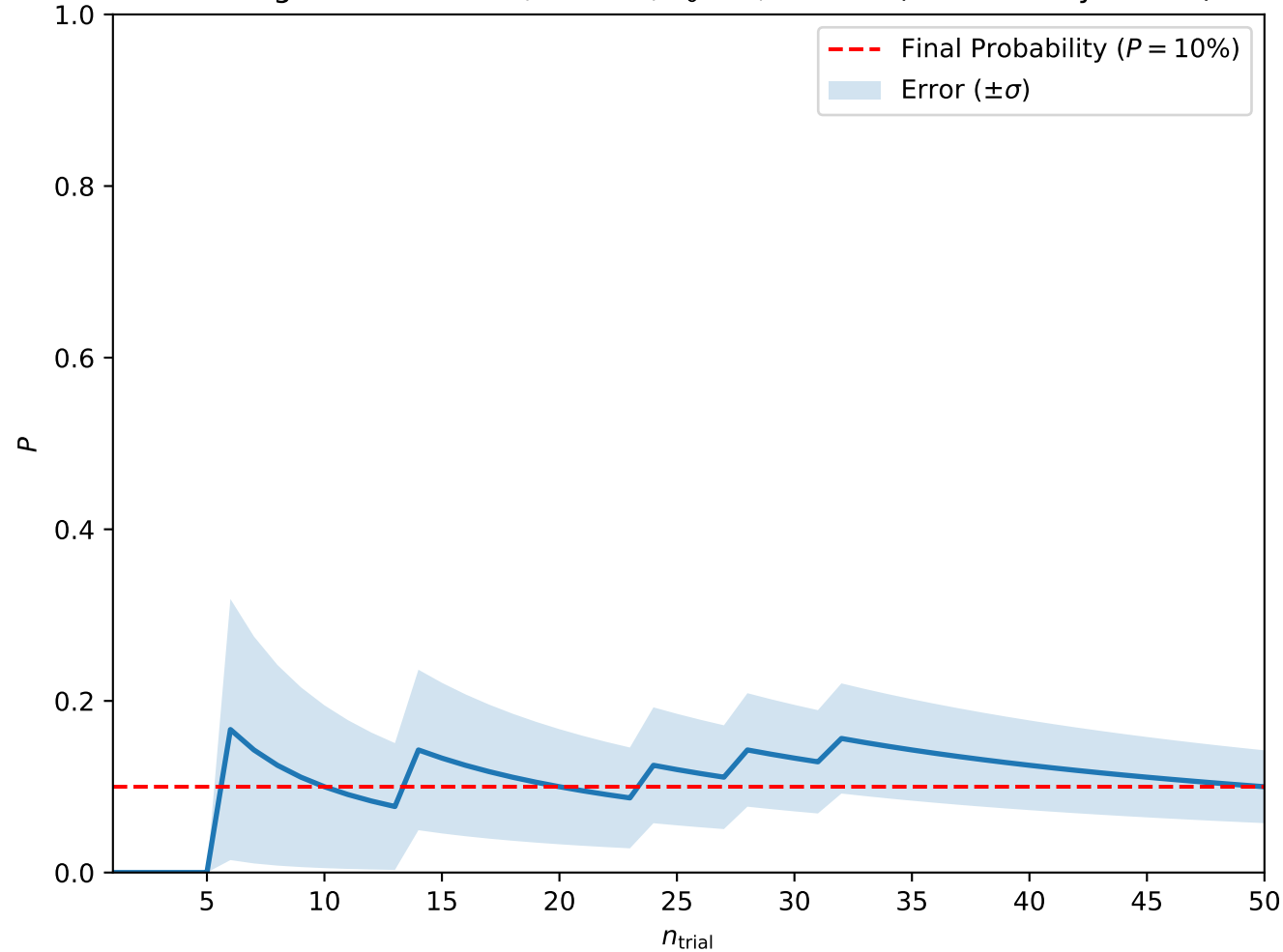
Convergence at A = 0.7, H = 0.3, T_0 = 3, w = 2.5 (Isolated Skyrmions)
