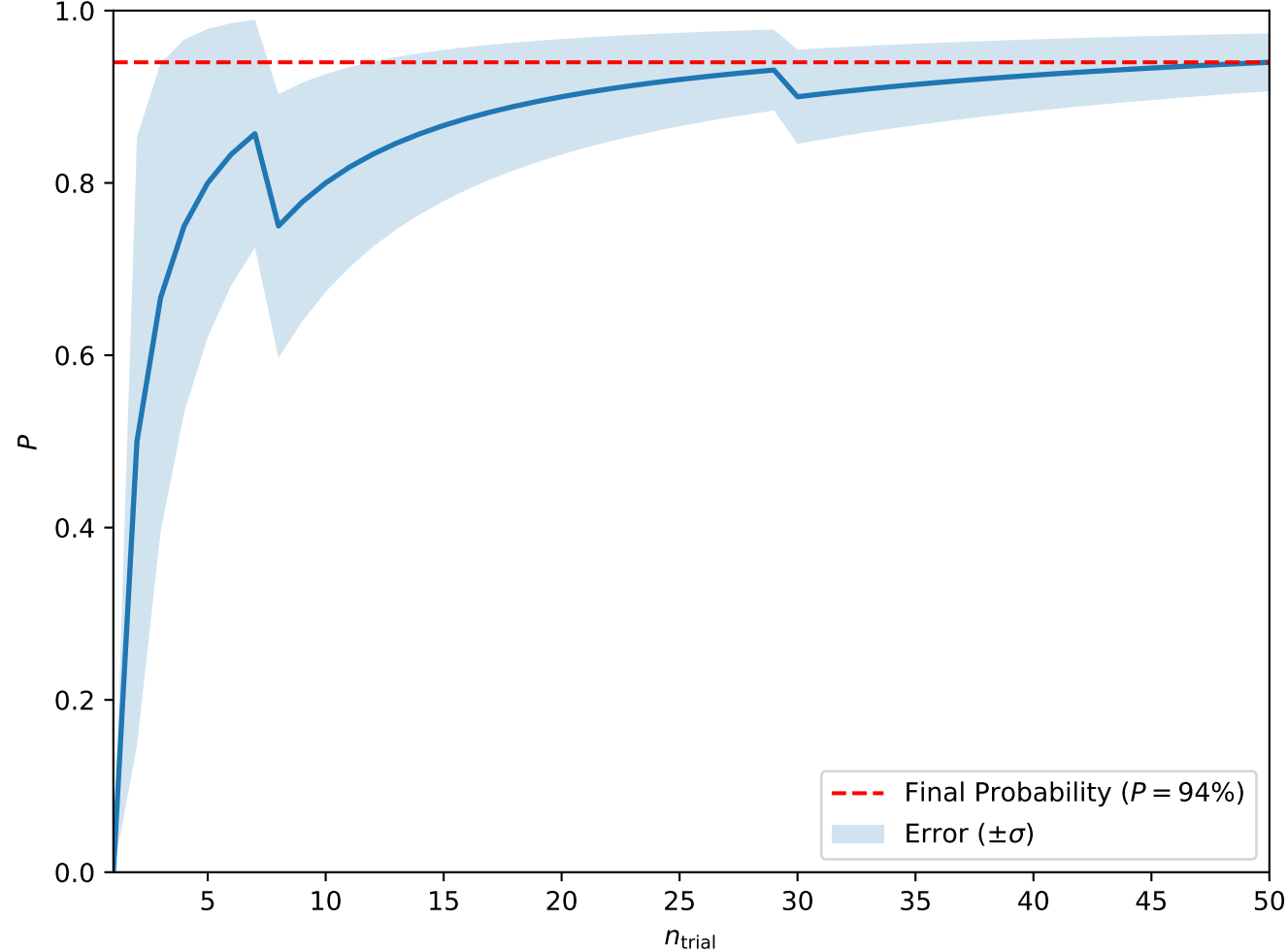
Convergence at A = 0.7, H = 0.3, T_0 = 3, w = 5 (Isolated Skyrmions)
