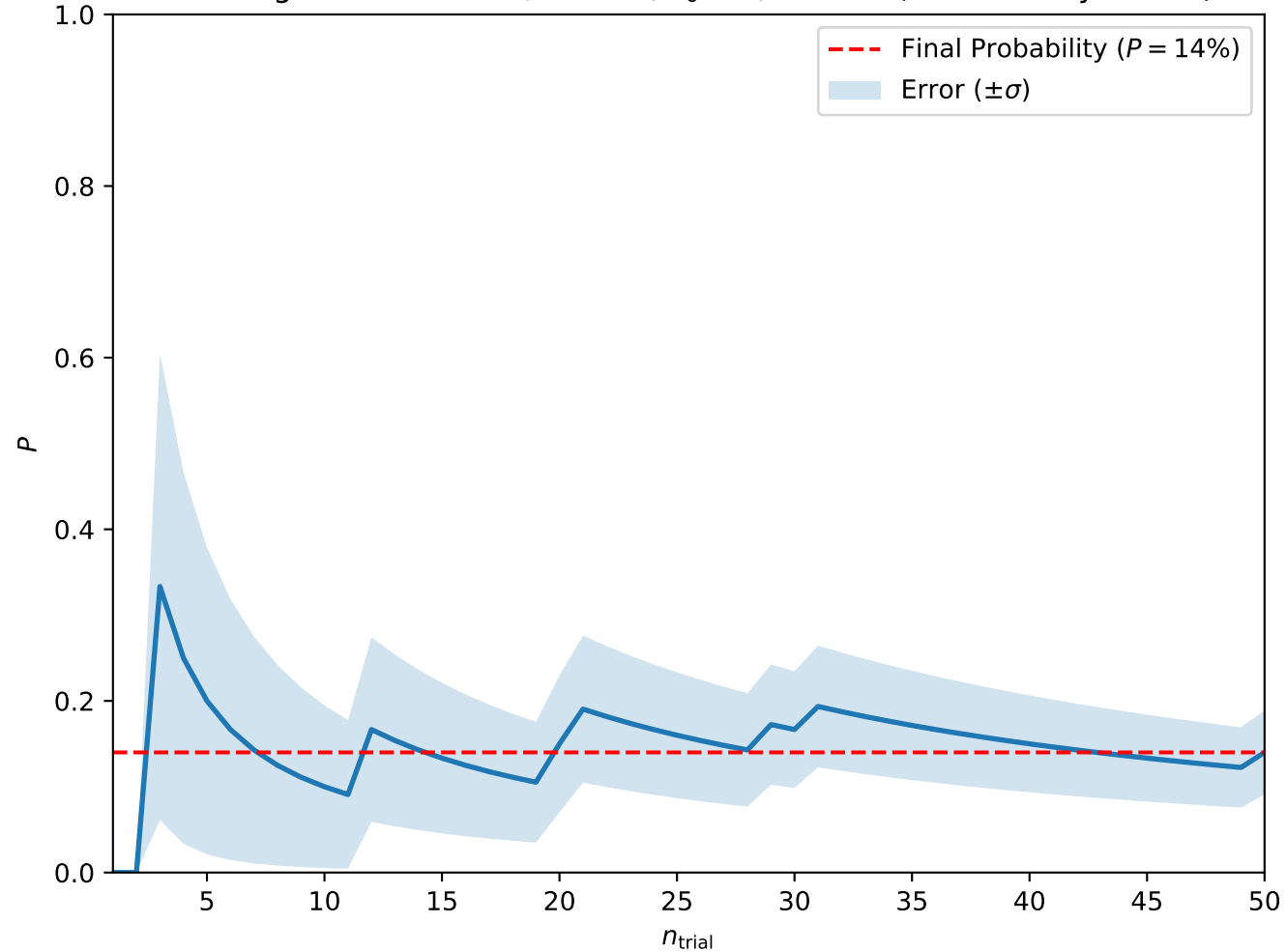
Convergence at A = 0.7, H = 0.3, T_0 = 5, w = 2.5 (Isolated Skyrmions)
