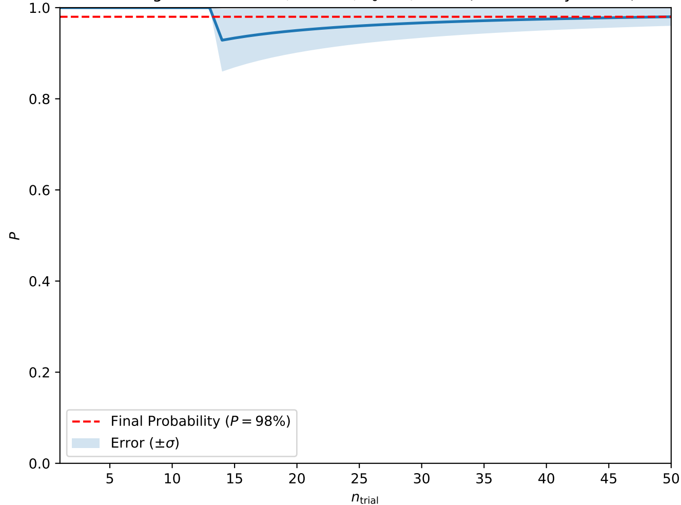
Convergence at A = 0.7, H = 0.3, T_0 = 5, w = 5 (Isolated Skyrmions)
