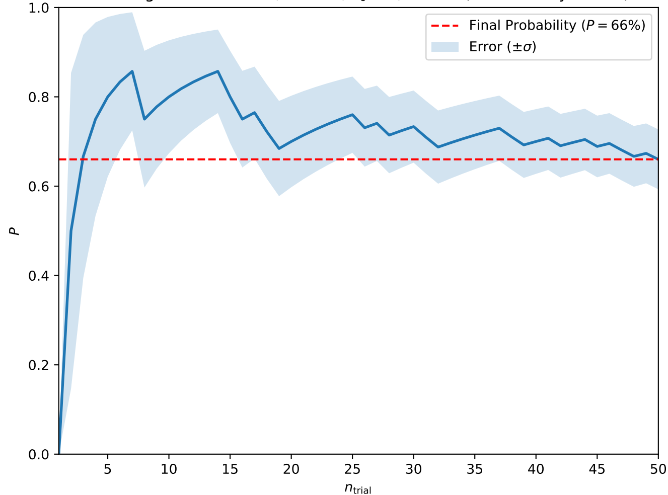
Convergence at A = 0.7, H = 0.4, T_0 = 1, w = 10 (Isolated Skyrmions)
