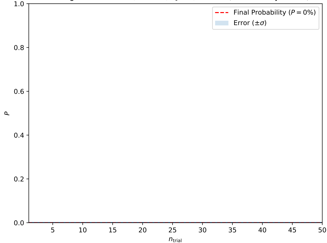
Convergence at A = 0.7, H = 0.4, T_0 = 1, w = 2.5 (Isolated Skyrmions)
