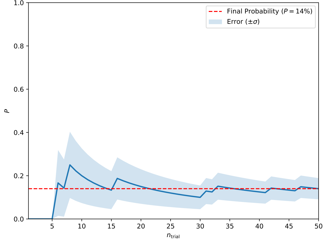
Convergence at A = 0.7, H = 0.4, T_0 = 1, w = 7.5 (Isolated Skyrmions)
