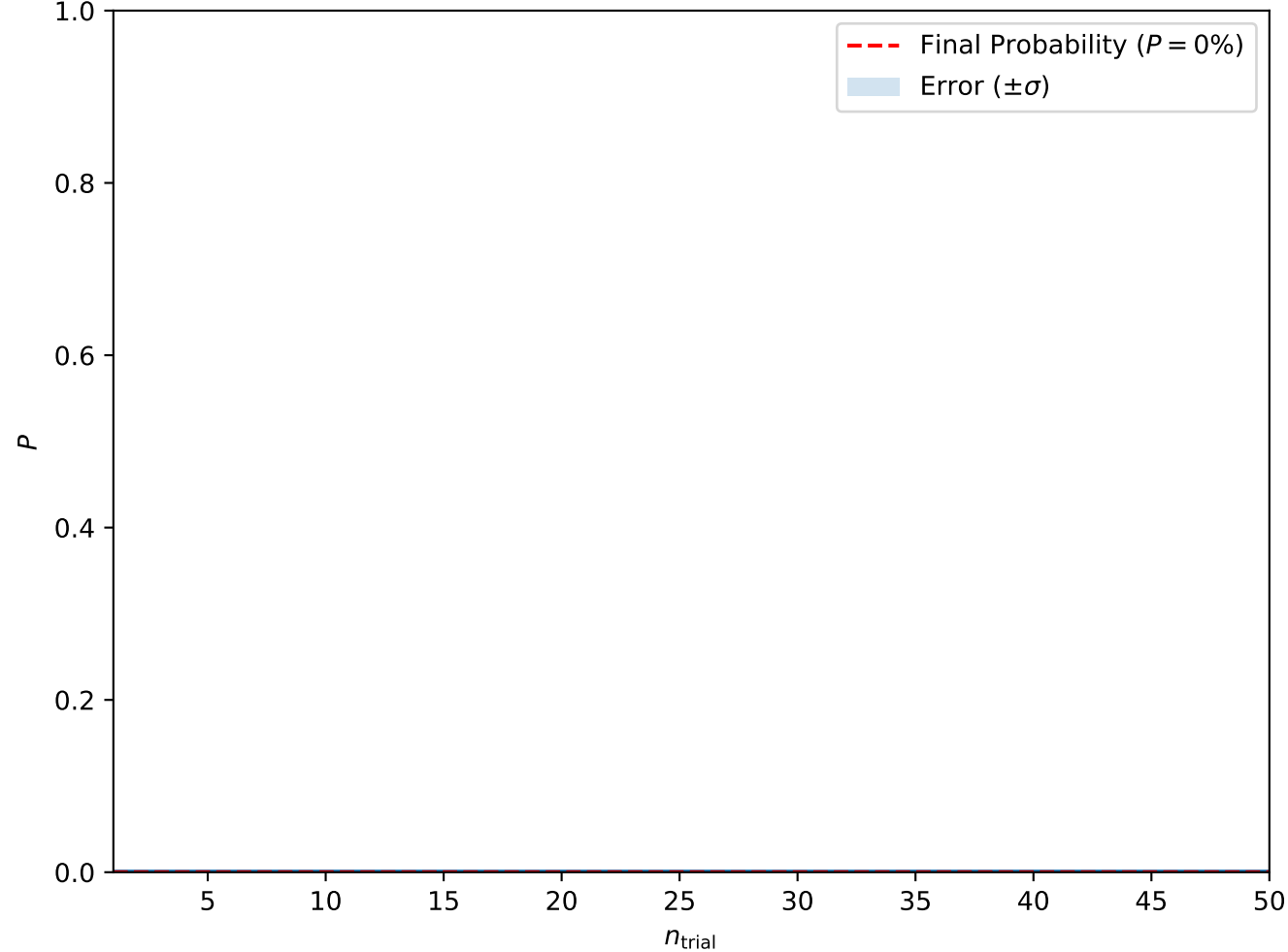
Convergence at A = 0.7, H = 0.4, T_0 = 3, w = 2.5 (Isolated Skyrmions)
