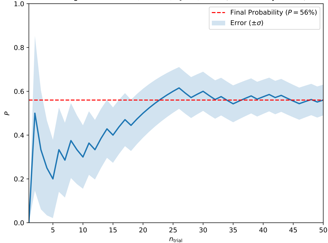
Convergence at A = 0.7, H = 0.4, T_0 = 3, w = 5 (Isolated Skyrmions)
