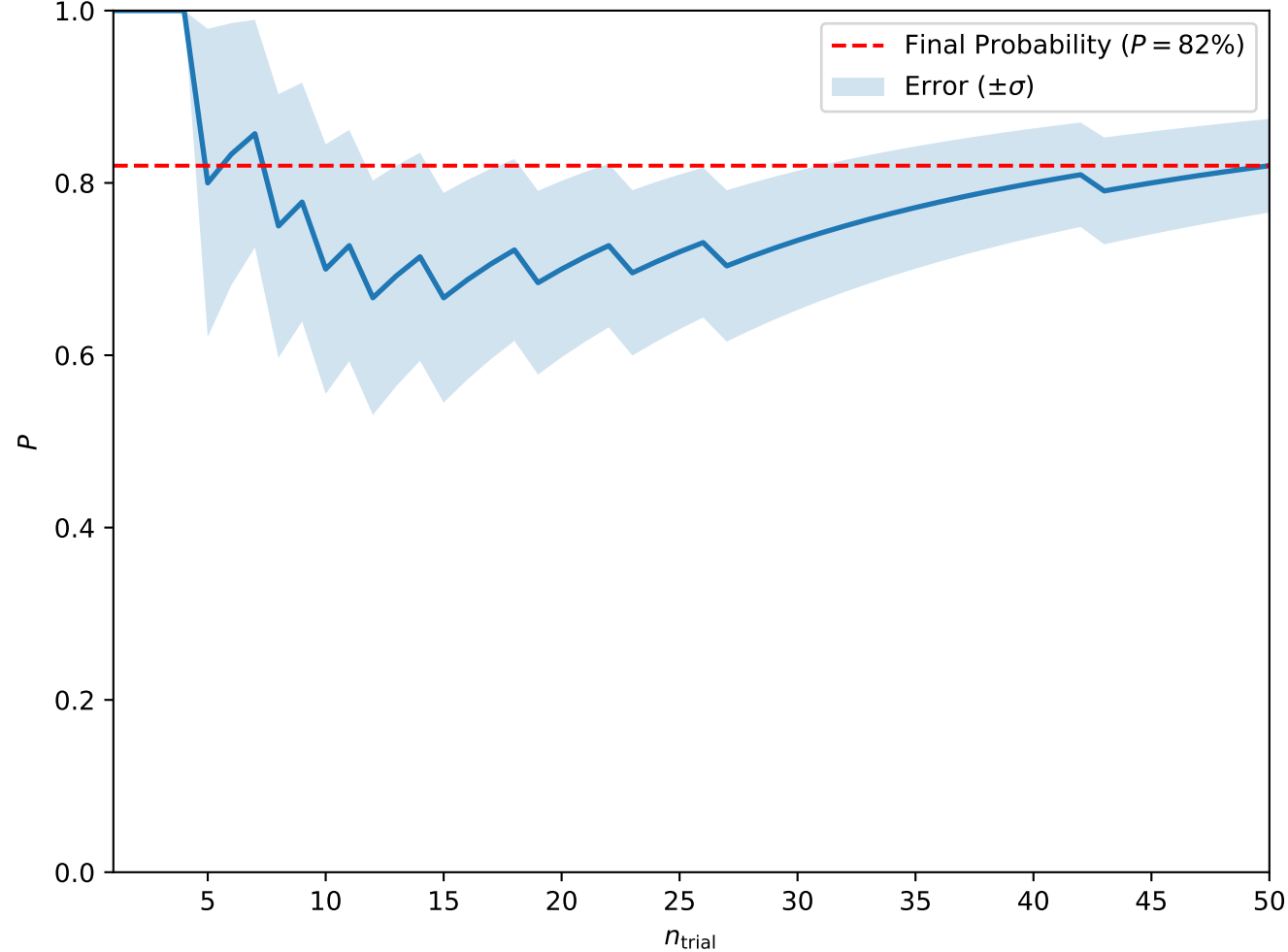
Convergence at A = 0.7, H = 0.4, T_0 = 3, w = 7.5 (Isolated Skyrmions)
