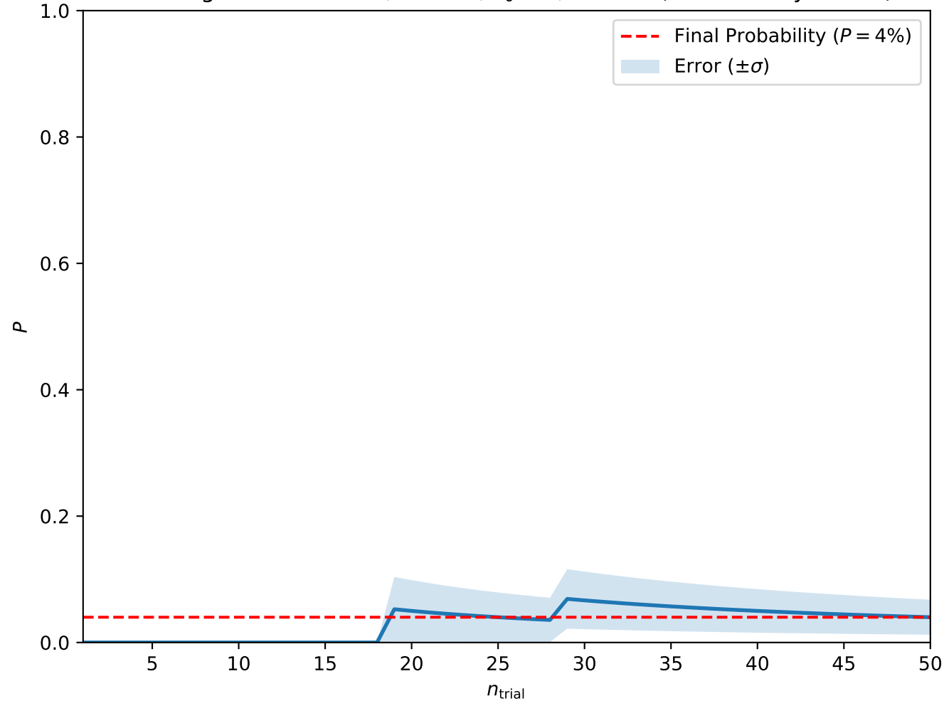
Convergence at A = 0.7, H = 0.4, T_0 = 5, w = 2.5 (Isolated Skyrmions)
