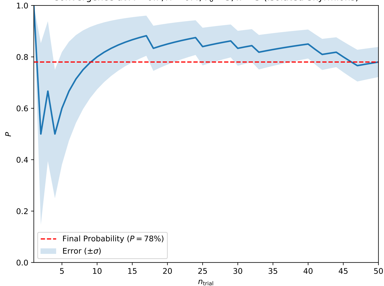
Convergence at A = 0.7, H = 0.4, T_0 = 5, w = 5 (Isolated Skyrmions)
