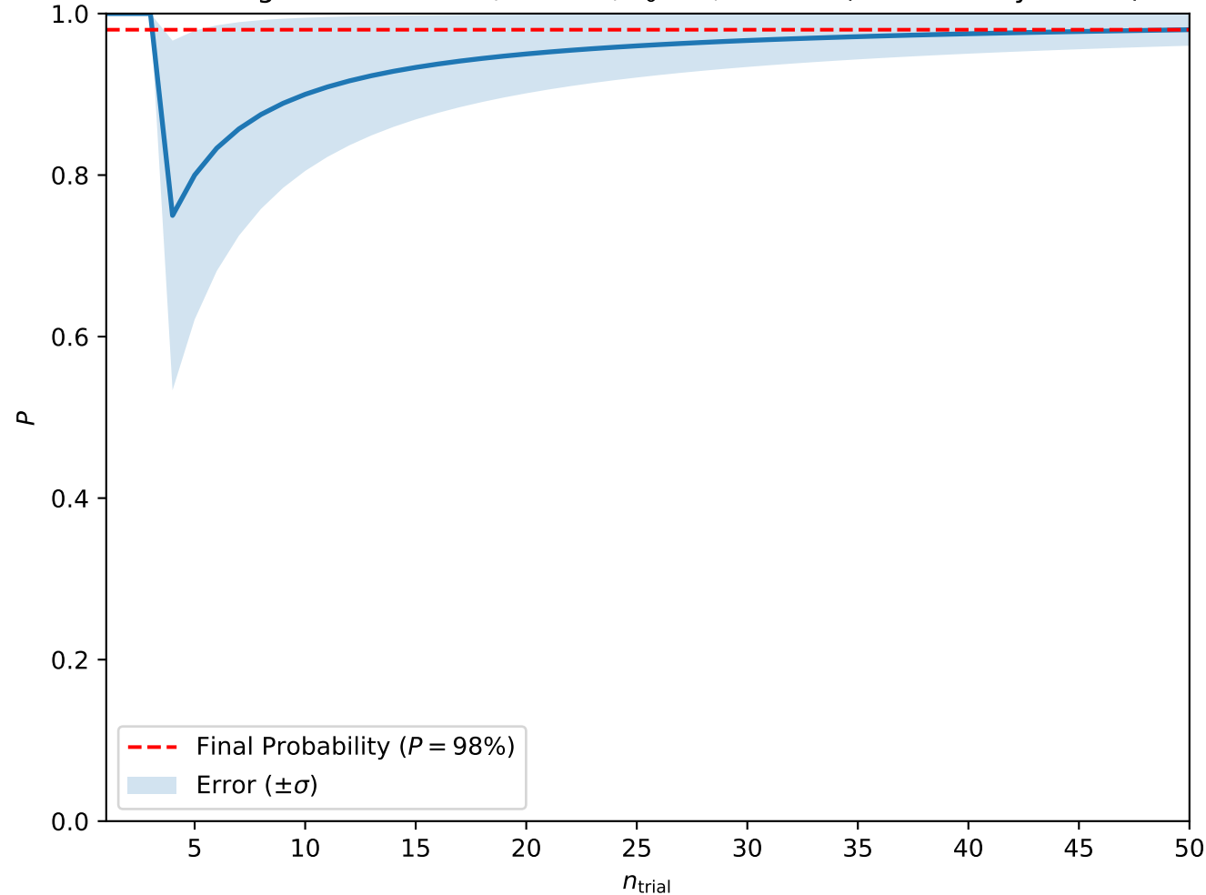
Convergence at A = 0.7, H = 0.4, T_0 = 5, w = 7.5 (Isolated Skyrmions)
