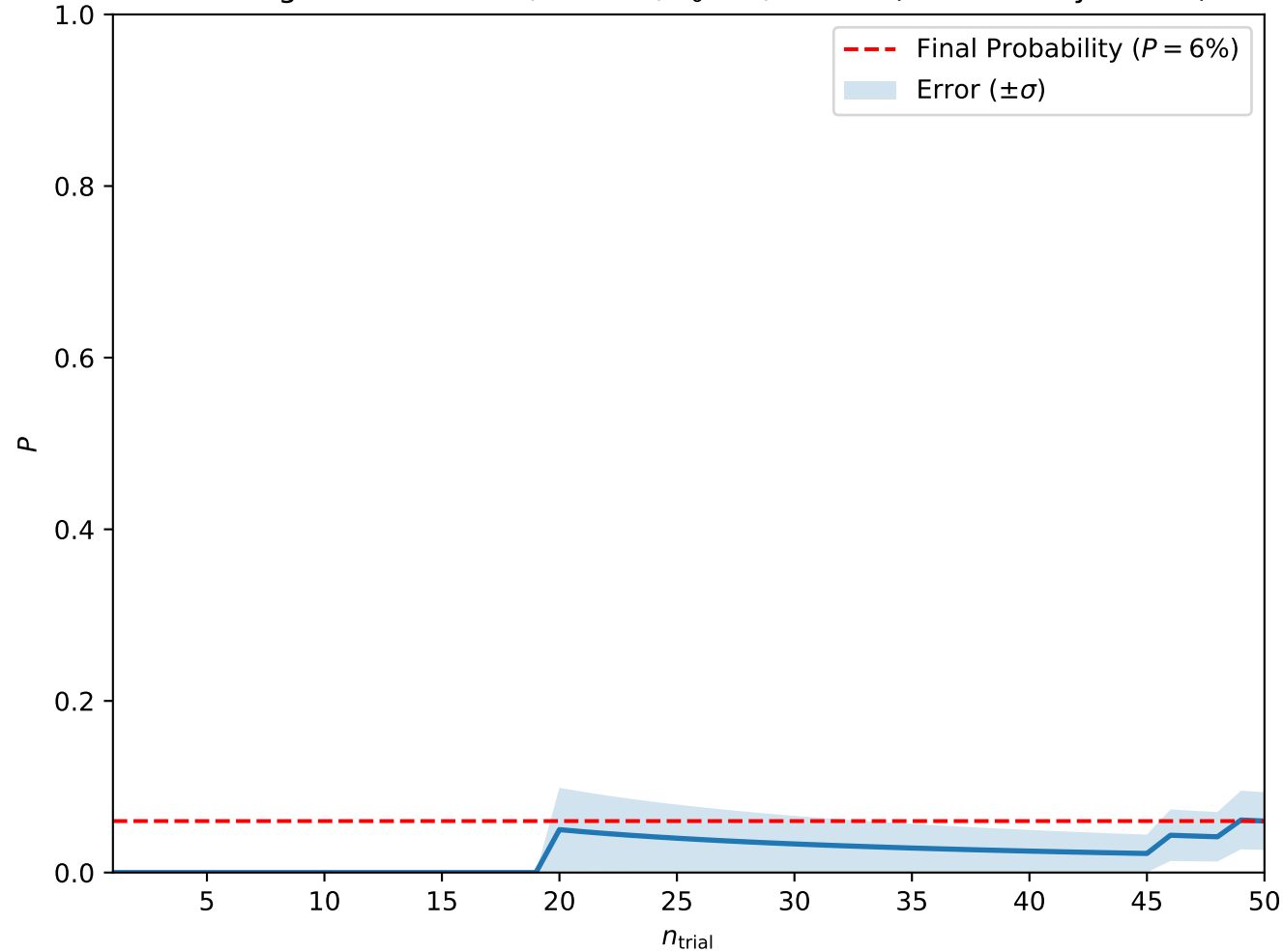
Convergence at A = 0.7, H = 0.5, T_0 = 1, w = 10 (Isolated Skyrmions)
