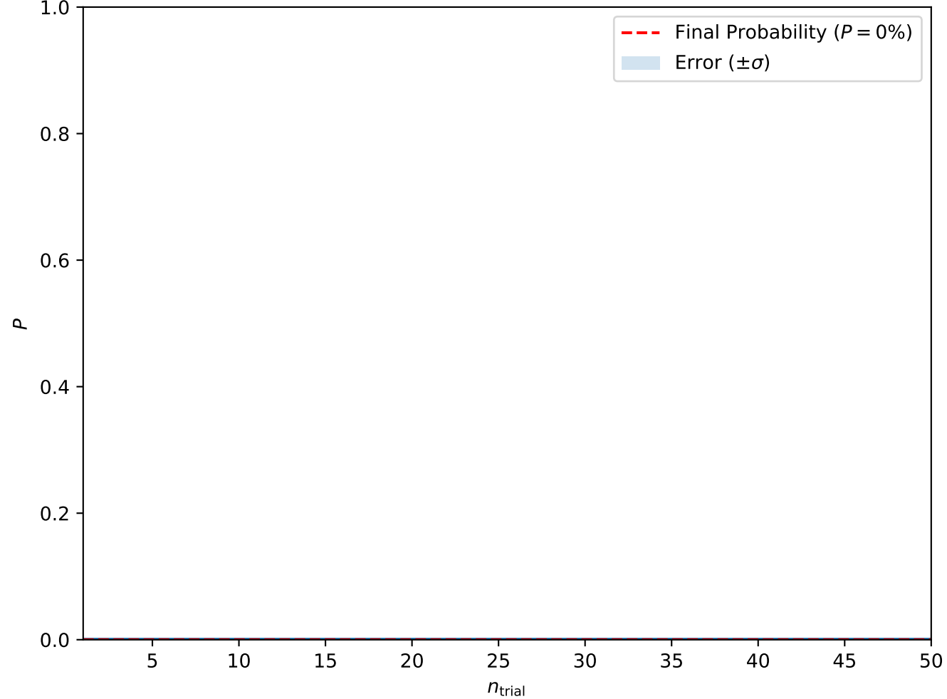
Convergence at A = 0.7, H = 0.5, T_0 = 1, w = 5 (Isolated Skyrmions)
